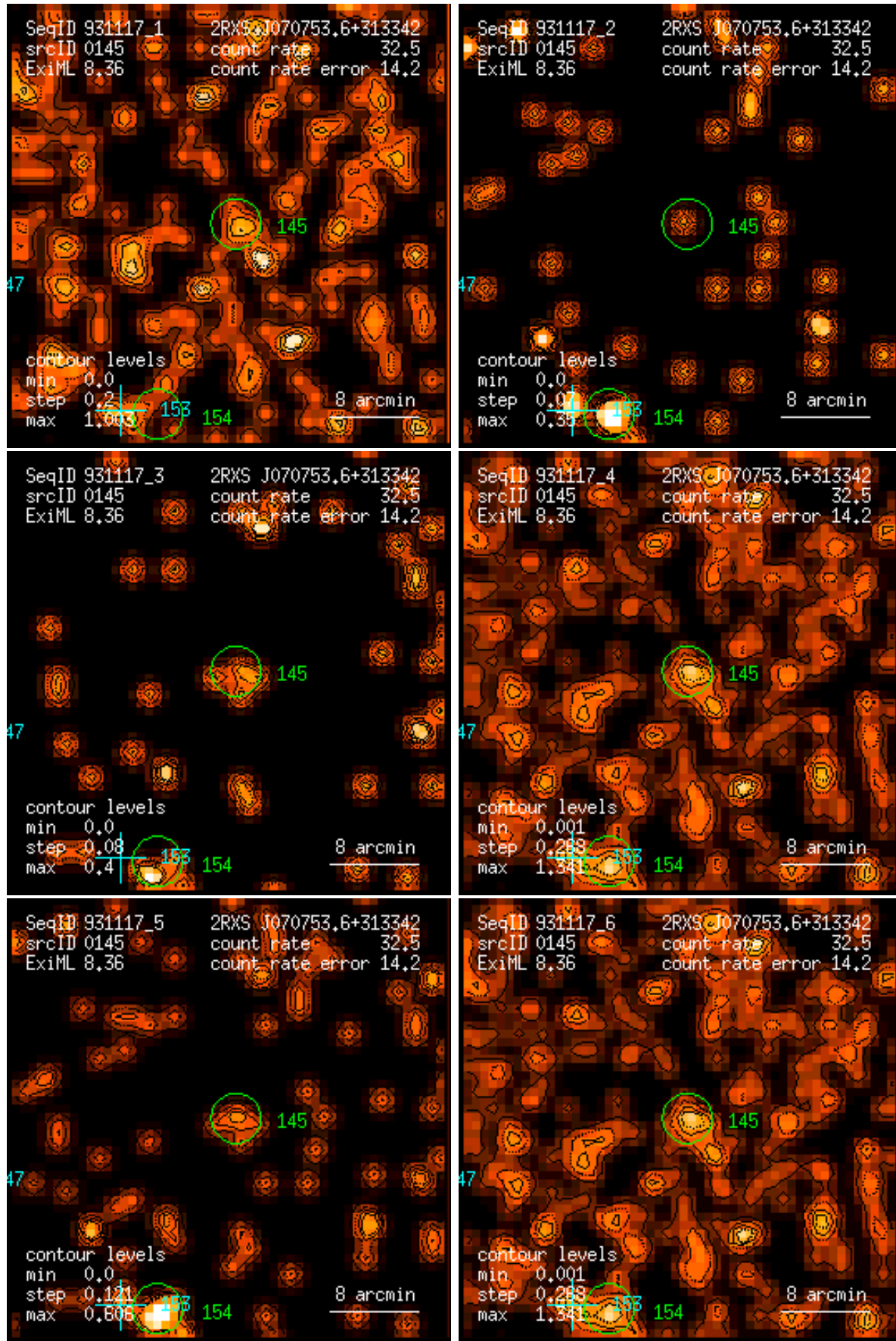
Figure 145: RASS 931117: detection 0145: band rate images, Gaussian filter: (1) PSPC channels 11 – 41, (2) 52 – 90, (3) 91 – 201, (4) 11 – 235, (5) 52 – 201, (6) 11 – 201. Broad band rates in counts/ks. Band rate contour levels in counts/ks/arcmin 2 .
