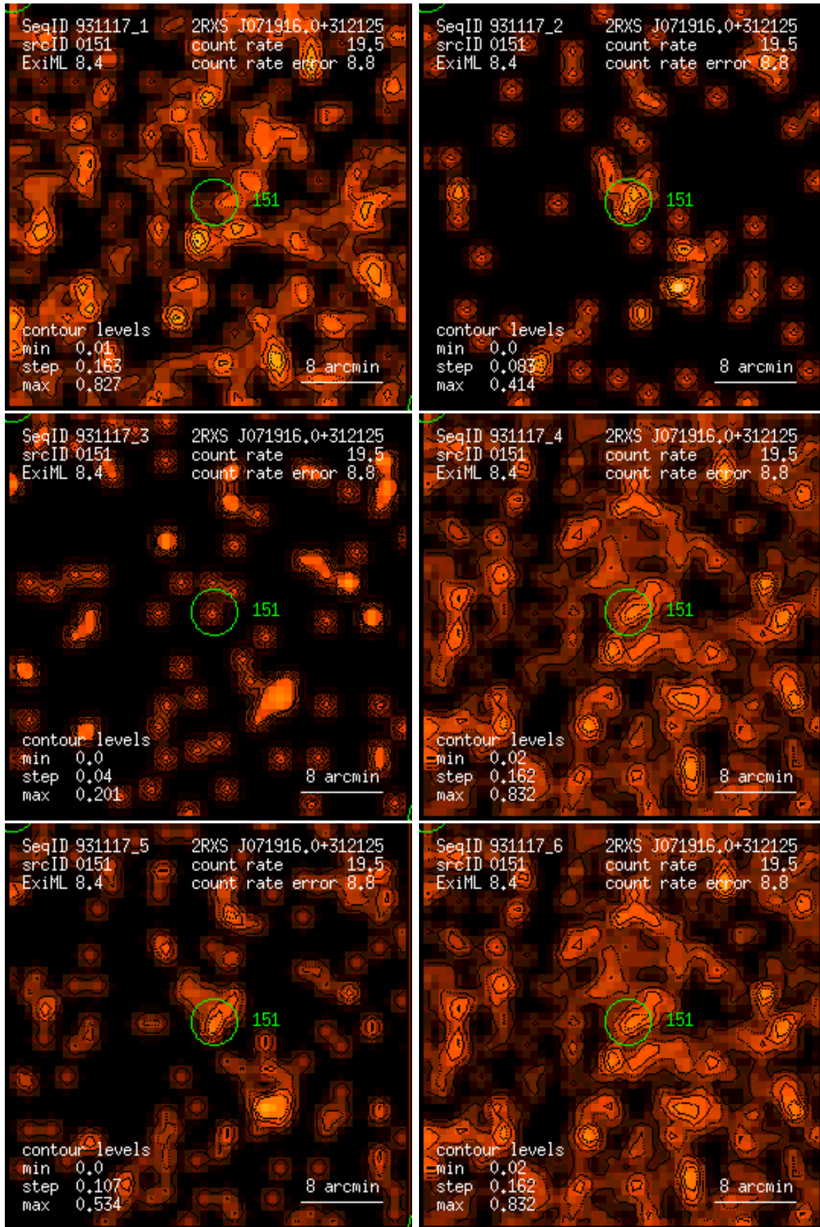
Figure 151: RASS 931117: detection 0151: band rate images, Gaussian filter: (1) PSPC channels 11 – 41, (2) 52 – 90, (3) 91 – 201, (4) 11 – 235, (5) 52 – 201, (6) 11 – 201. Broad band rates in counts/ks. Band rate contour levels in counts/ks/arcmin 2 .
