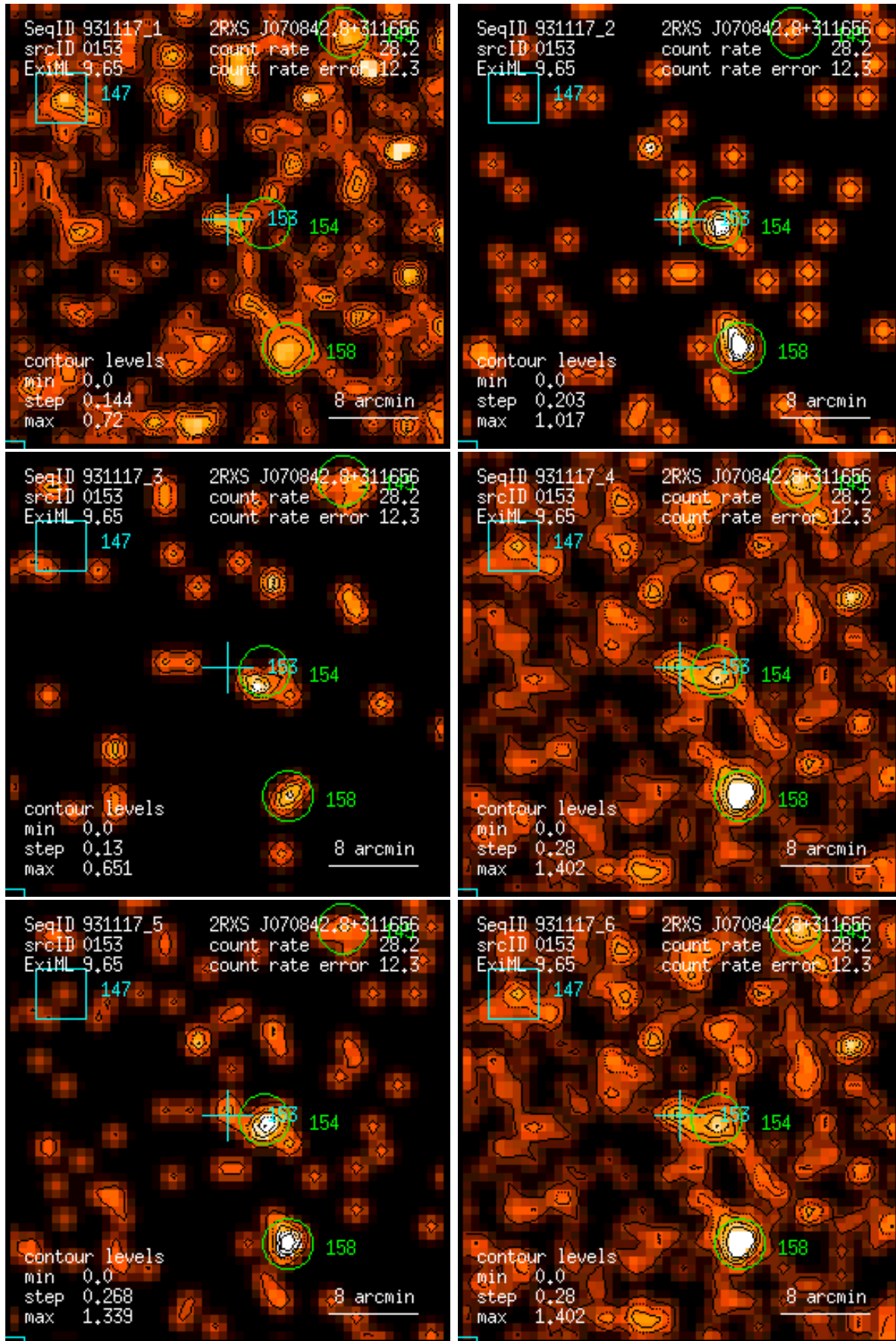
Figure 153: RASS 931117: detection 0153: band rate images, Gaussian filter: (1) PSPC channels 11 – 41, (2) 52 – 90, (3) 91 – 201, (4) 11 – 235, (5) 52 – 201, (6) 11 – 201. Broad band rates in counts/ks. Band rate contour levels in counts/ks/arcmin 2 .
