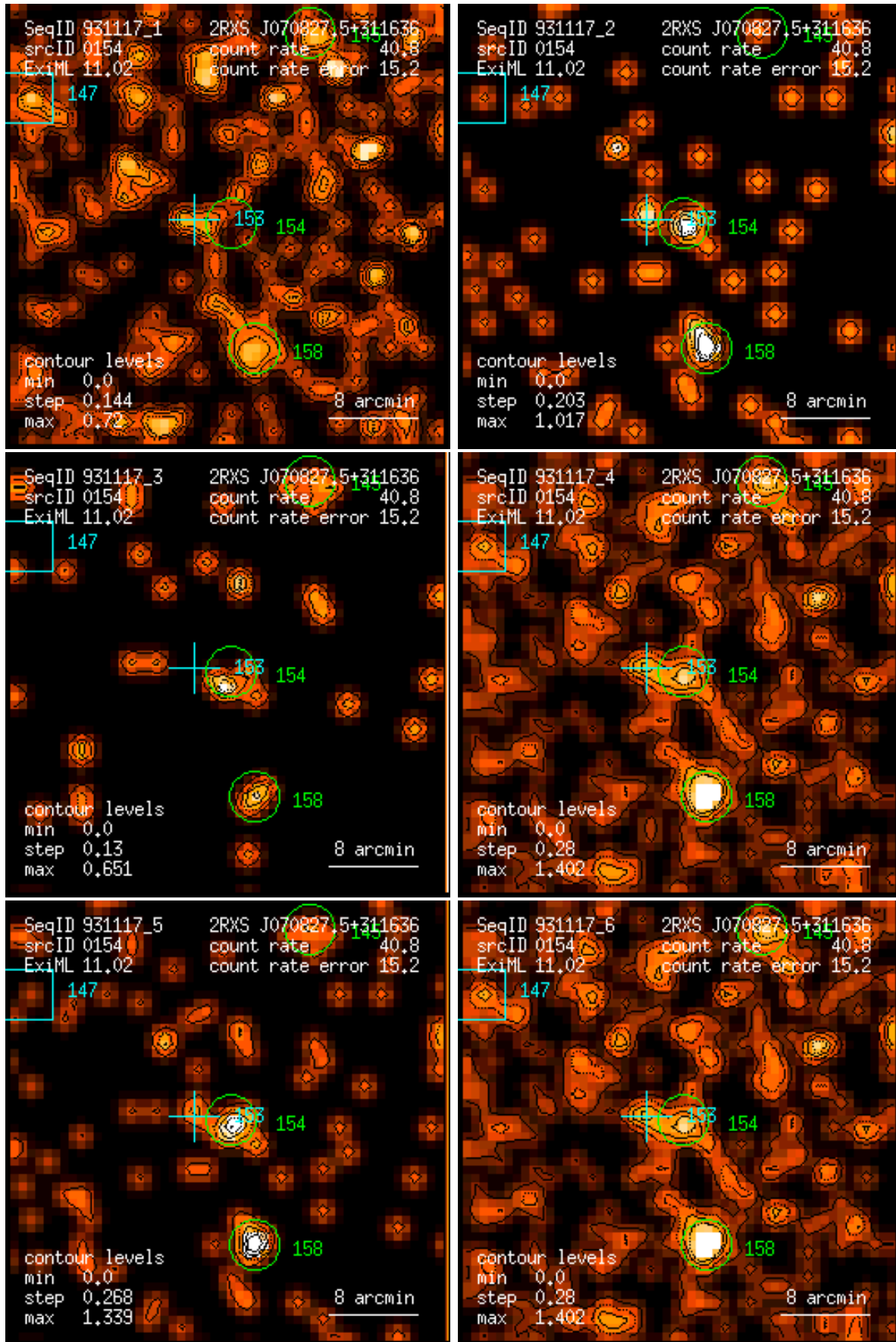
Figure 154: RASS 931117: detection 0154: band rate images, Gaussian filter: (1) PSPC channels 11 – 41, (2) 52 – 90, (3) 91 – 201, (4) 11 – 235, (5) 52 – 201, (6) 11 – 201. Broad band rates in counts/ks. Band rate contour levels in counts/ks/arcmin 2 .
