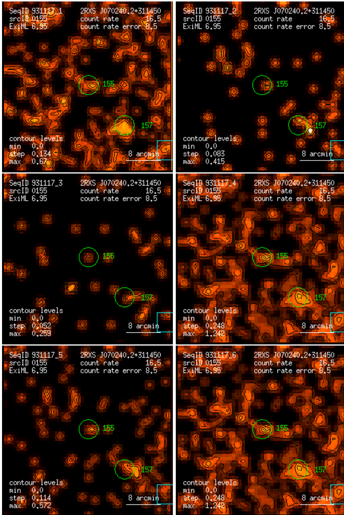
Figure 155: RASS 931117: detection 0155: band rate images, Gaussian filter: (1) PSPC channels 11 – 41, (2) 52 – 90, (3) 91 – 201, (4) 11 – 235, (5) 52 – 201, (6) 11 – 201. Broad band rates in counts/ks. Band rate contour levels in counts/ks/arcmin 2 .
