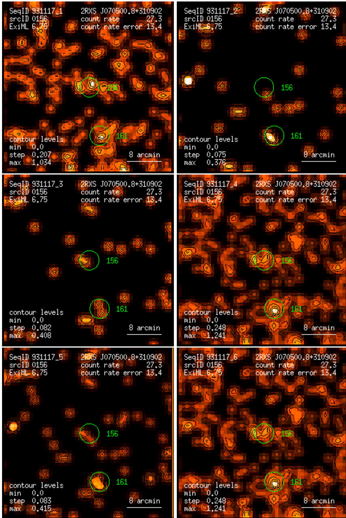
Figure 156: RASS 931117: detection 0156: band rate images, Gaussian filter: (1) PSPC channels 11 – 41, (2) 52 – 90, (3) 91 – 201, (4) 11 – 235, (5) 52 – 201, (6) 11 – 201. Broad band rates in counts/ks. Band rate contour levels in counts/ks/arcmin 2 .
