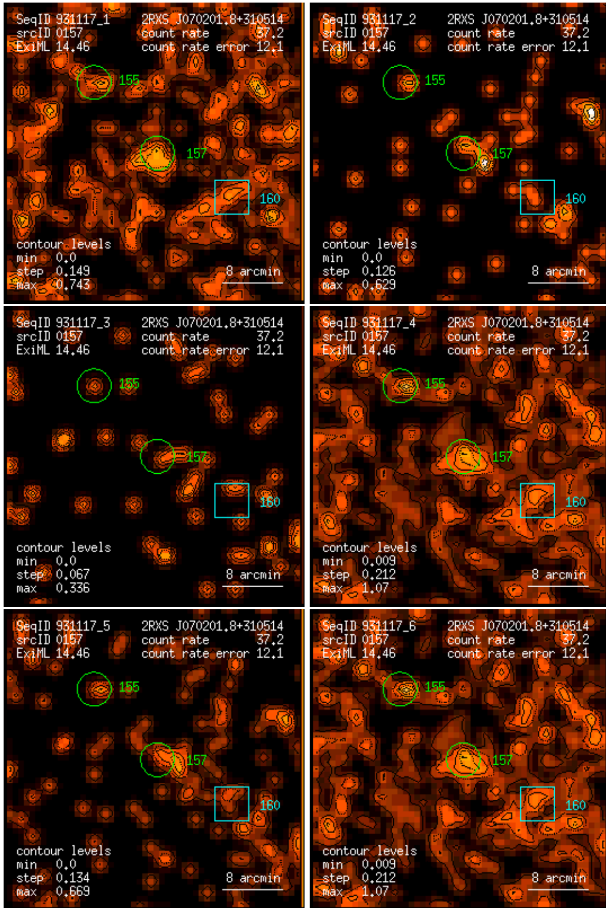
Figure 157: RASS 931117: detection 0157: band rate images, Gaussian filter: (1) PSPC channels 11 – 41, (2) 52 – 90, (3) 91 – 201, (4) 11 – 235, (5) 52 – 201, (6) 11 – 201. Broad band rates in counts/ks. Band rate contour levels in counts/ks/arcmin 2 .
