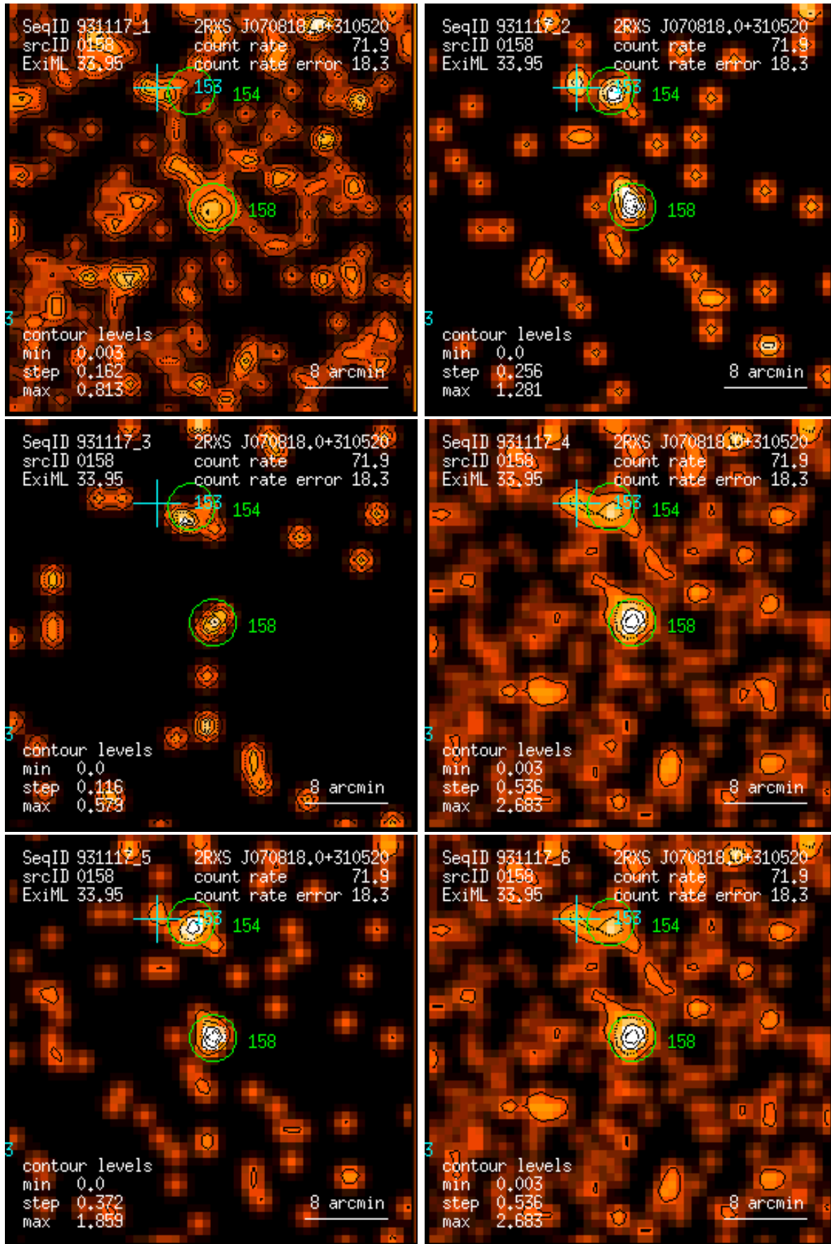
Figure 158: RASS 931117: detection 0158: band rate images, Gaussian filter: (1) PSPC channels 11 – 41, (2) 52 – 90, (3) 91 – 201, (4) 11 – 235, (5) 52 – 201, (6) 11 – 201. Broad band rates in counts/ks. Band rate contour levels in counts/ks/arcmin 2 .
