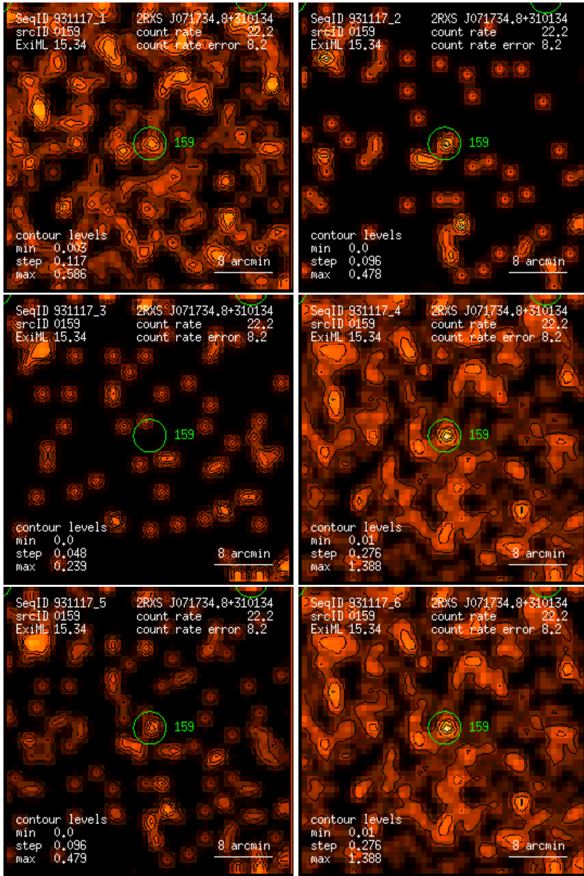
Figure 159: RASS 931117: detection 0159: band rate images, Gaussian filter: (1) PSPC channels 11 – 41, (2) 52 – 90, (3) 91 – 201, (4) 11 – 235, (5) 52 – 201, (6) 11 – 201. Broad band rates in counts/ks. Band rate contour levels in counts/ks/arcmin 2 .
