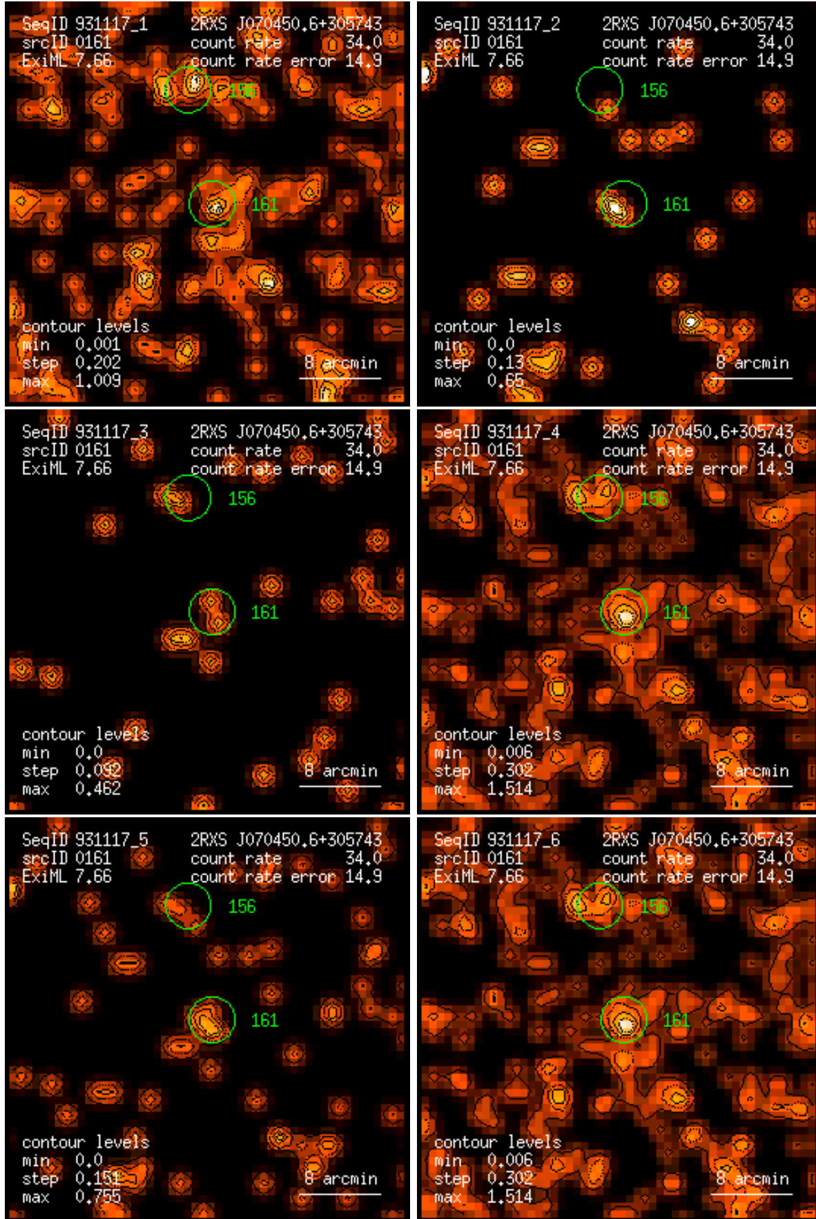
Figure 161: RASS 931117: detection 0161: band rate images, Gaussian filter: (1) PSPC channels 11 – 41, (2) 52 – 90, (3) 91 – 201, (4) 11 – 235, (5) 52 – 201, (6) 11 – 201. Broad band rates in counts/ks. Band rate contour levels in counts/ks/arcmin 2 .
