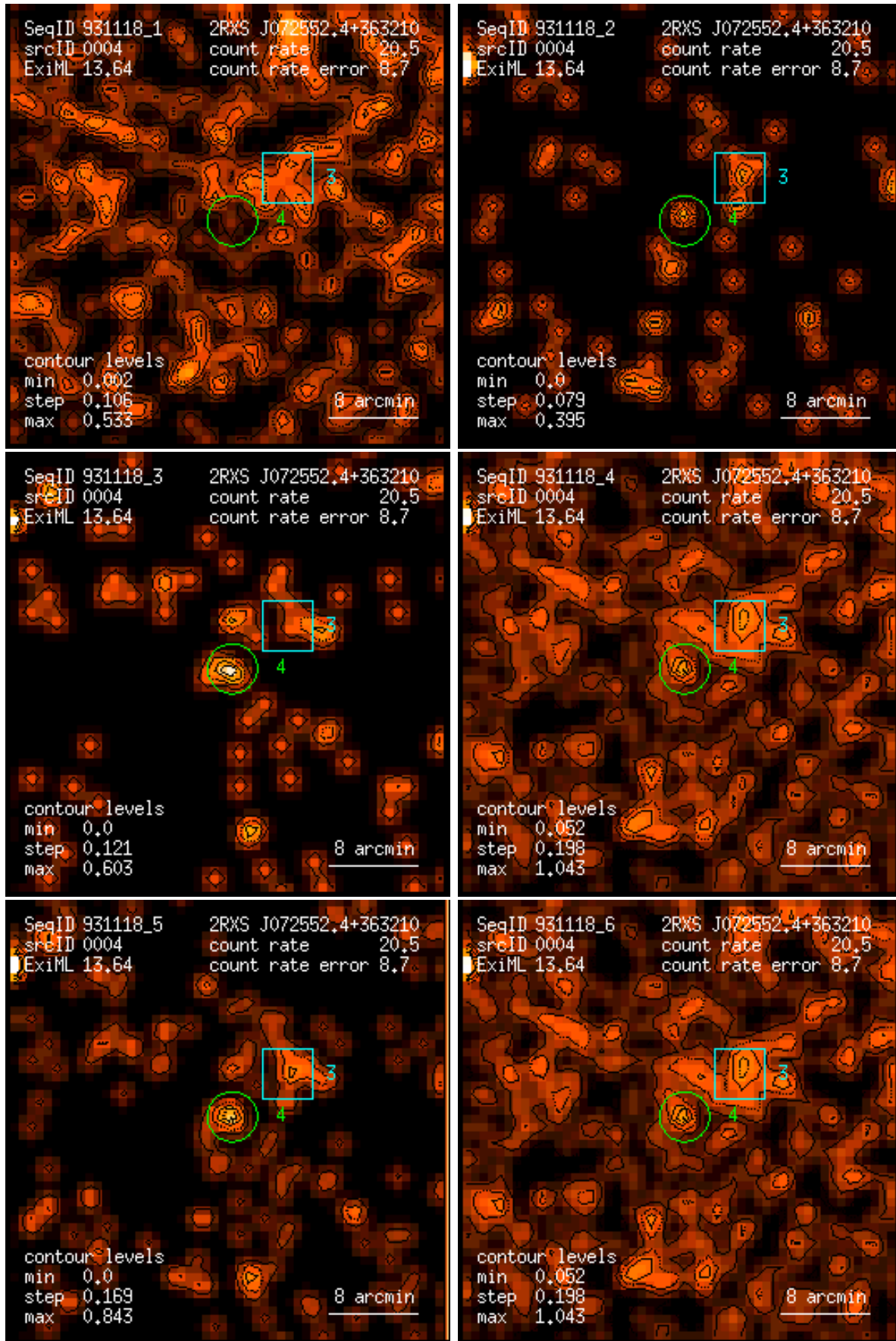
Figure 4: RASS 931118: detection 0004: band rate images, Gaussian filter: (1) PSPC channels 11 – 41, (2) 52 – 90, (3) 91 – 201, (4) 11 – 235, (5) 52 – 201, (6) 11 – 201. Broad band rates in counts/ks. Band rate contour levels in counts/ks/arcmin 2 .
