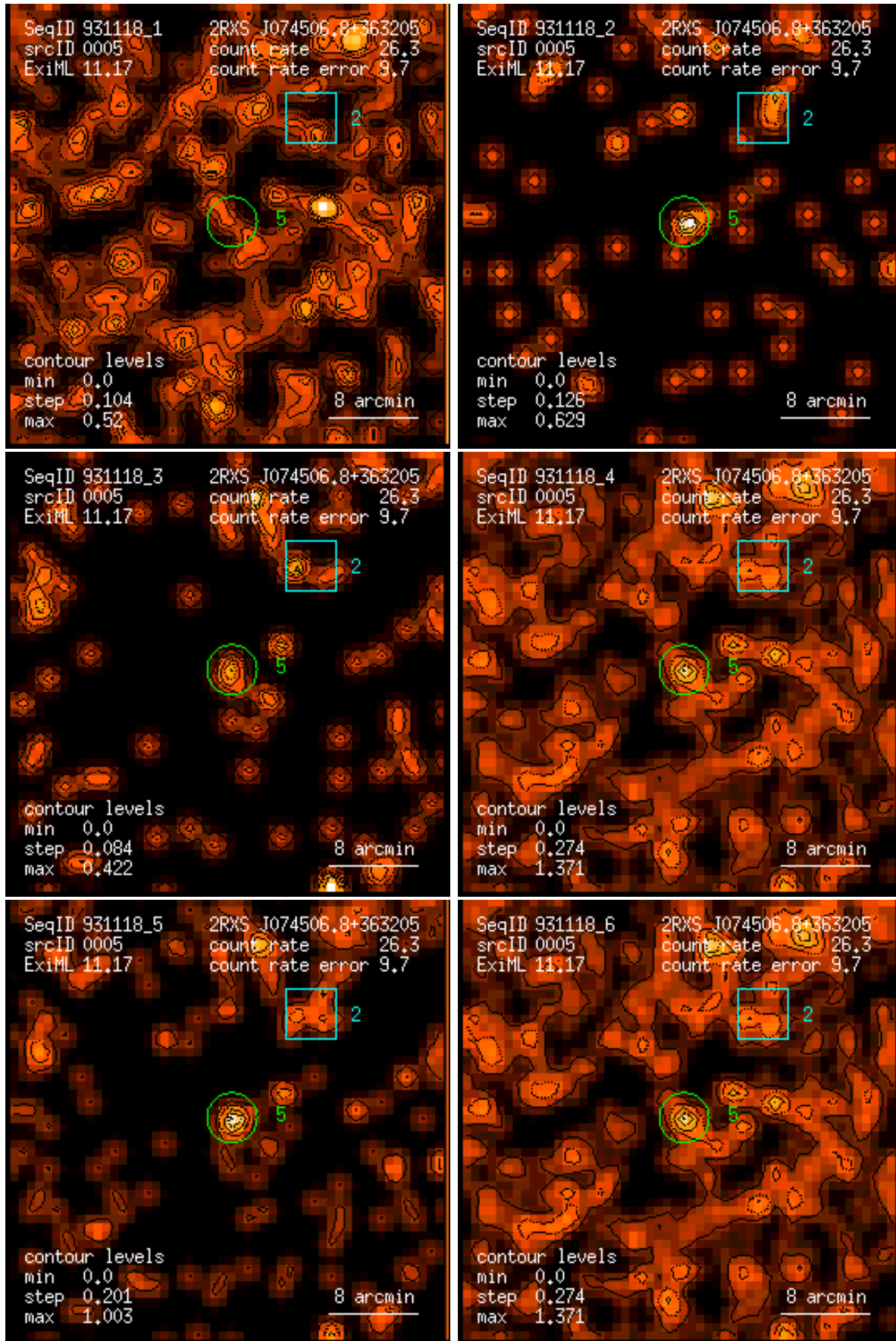
Figure 5: RASS 931118: detection 0005: band rate images, Gaussian filter: (1) PSPC channels 11 – 41, (2) 52 – 90, (3) 91 – 201, (4) 11 – 235, (5) 52 – 201, (6) 11 – 201. Broad band rates in counts/ks. Band rate contour levels in counts/ks/arcmin 2 .
