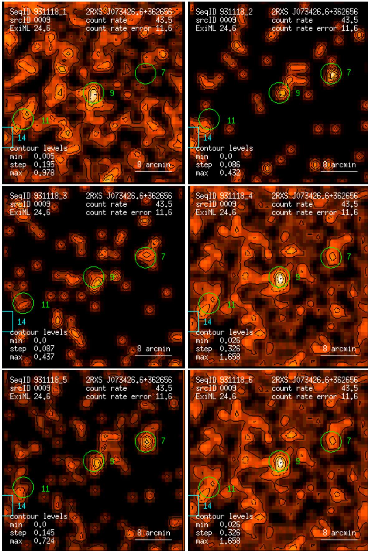
Figure 9: RASS 931118: detection 0009: band rate images, Gaussian filter: (1) PSPC channels 11 – 41, (2) 52 – 90, (3) 91 – 201, (4) 11 – 235, (5) 52 – 201, (6) 11 – 201. Broad band rates in counts/ks. Band rate contour levels in counts/ks/arcmin 2 .
