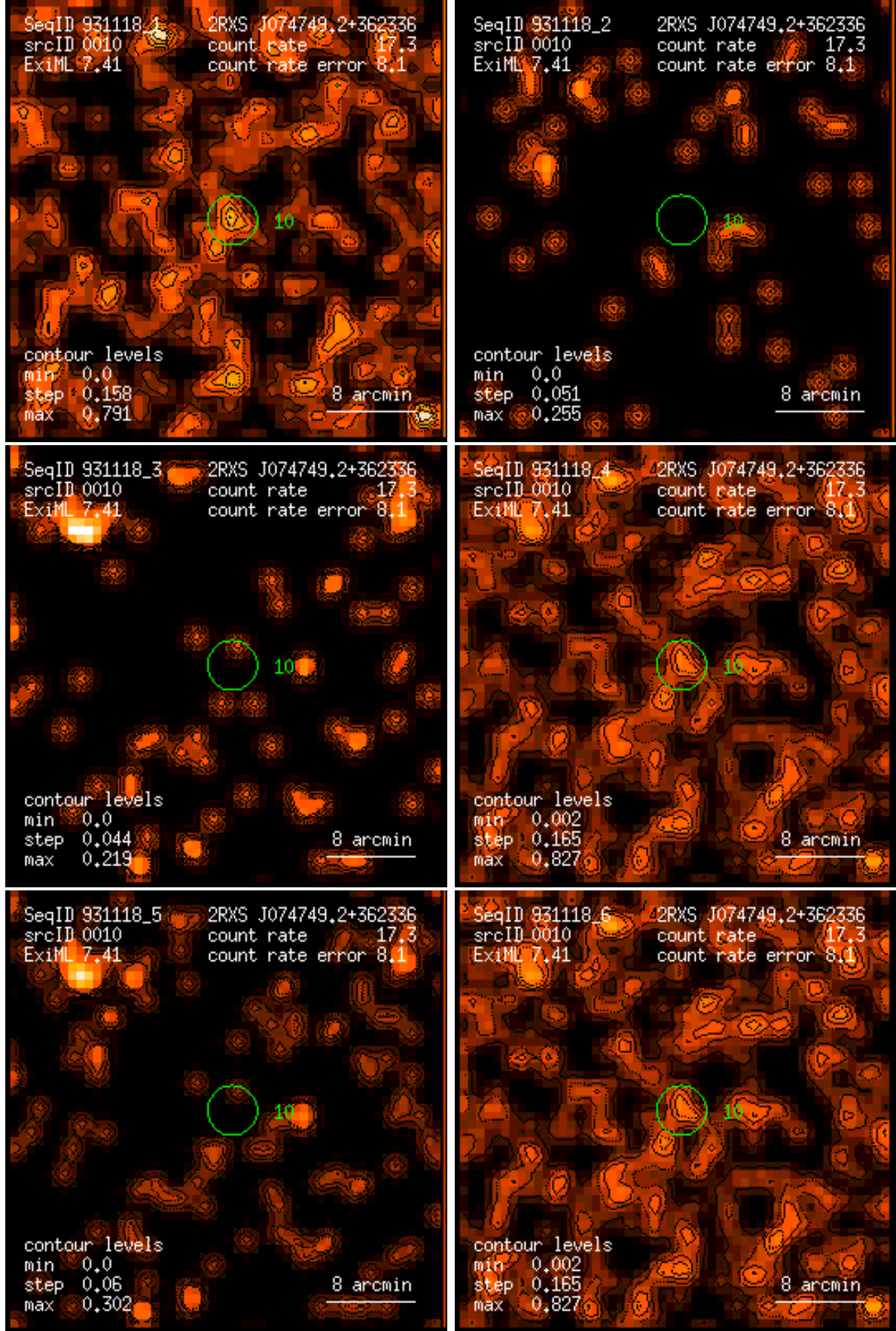
Figure 10: RASS 931118: detection 0010: band rate images, Gaussian filter: (1) PSPC channels 11 – 41, (2) 52 – 90, (3) 91 – 201, (4) 11 – 235, (5) 52 – 201, (6) 11 – 201. Broad band rates in counts/ks. Band rate contour levels in counts/ks/arcmin 2 .
