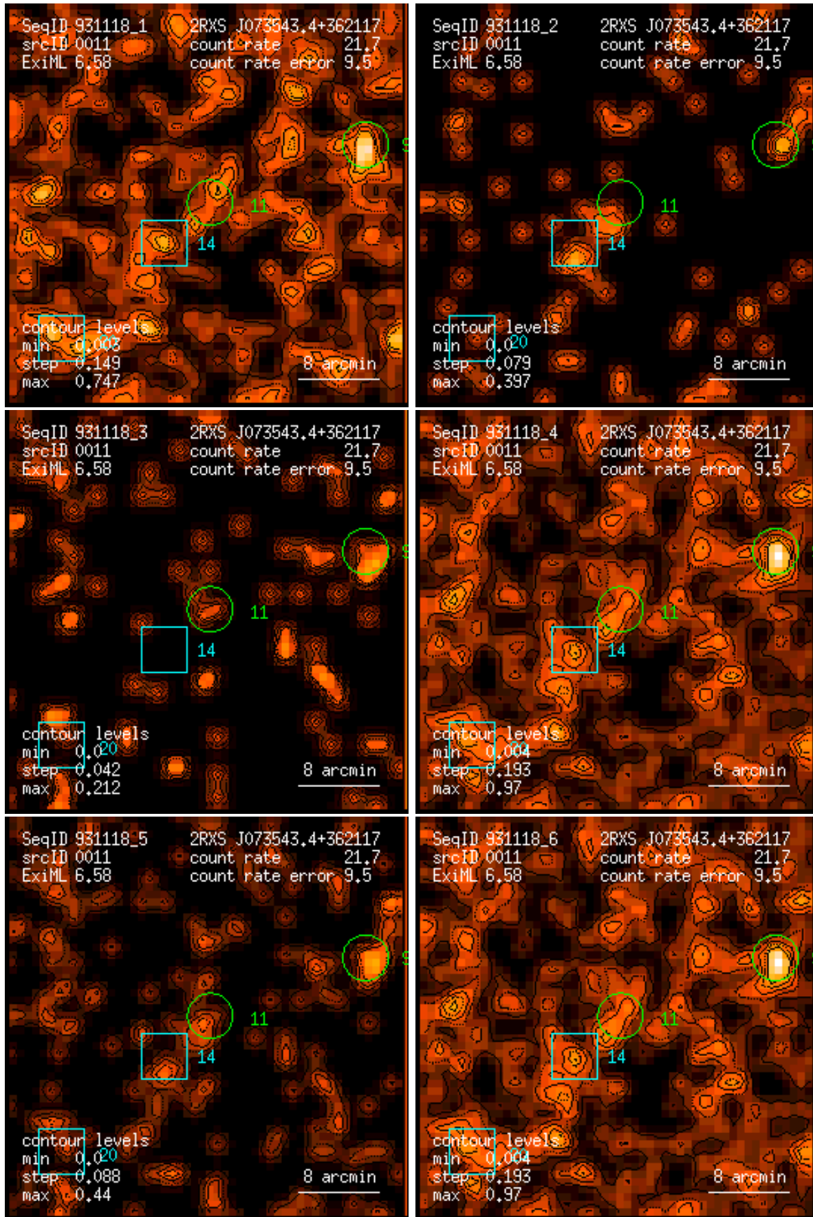
Figure 11: RASS 931118: detection 0011: band rate images, Gaussian filter: (1) PSPC channels 11 – 41, (2) 52 – 90, (3) 91 – 201, (4) 11 – 235, (5) 52 – 201, (6) 11 – 201. Broad band rates in counts/ks. Band rate contour levels in counts/ks/arcmin 2 .
