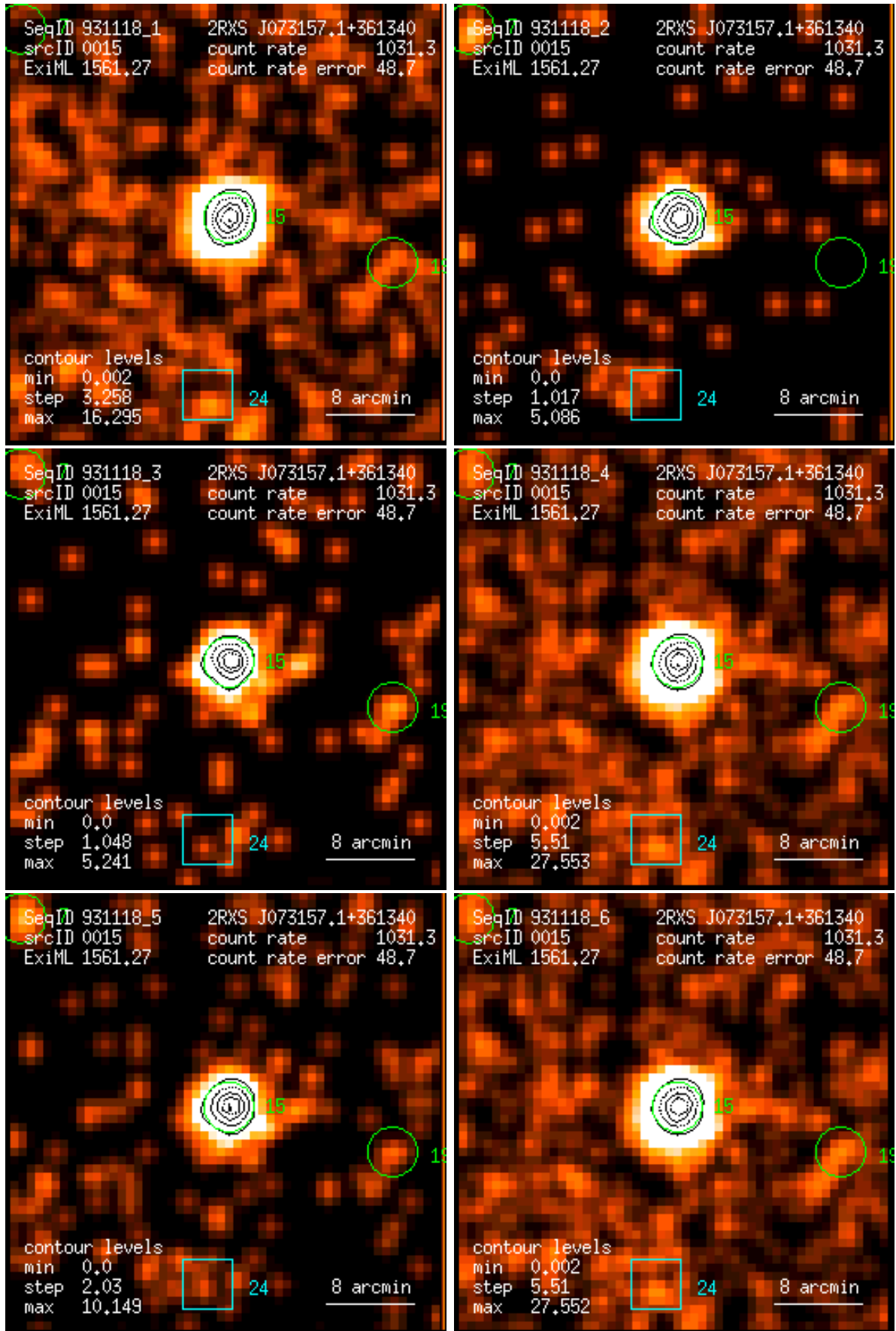
Figure 15: RASS 931118: detection 0015: band rate images, Gaussian filter: (1) PSPC channels 11 – 41, (2) 52 – 90, (3) 91 – 201, (4) 11 – 235, (5) 52 – 201, (6) 11 – 201. Broad band rates in counts/ks. Band rate contour levels in counts/ks/arcmin 2 .
