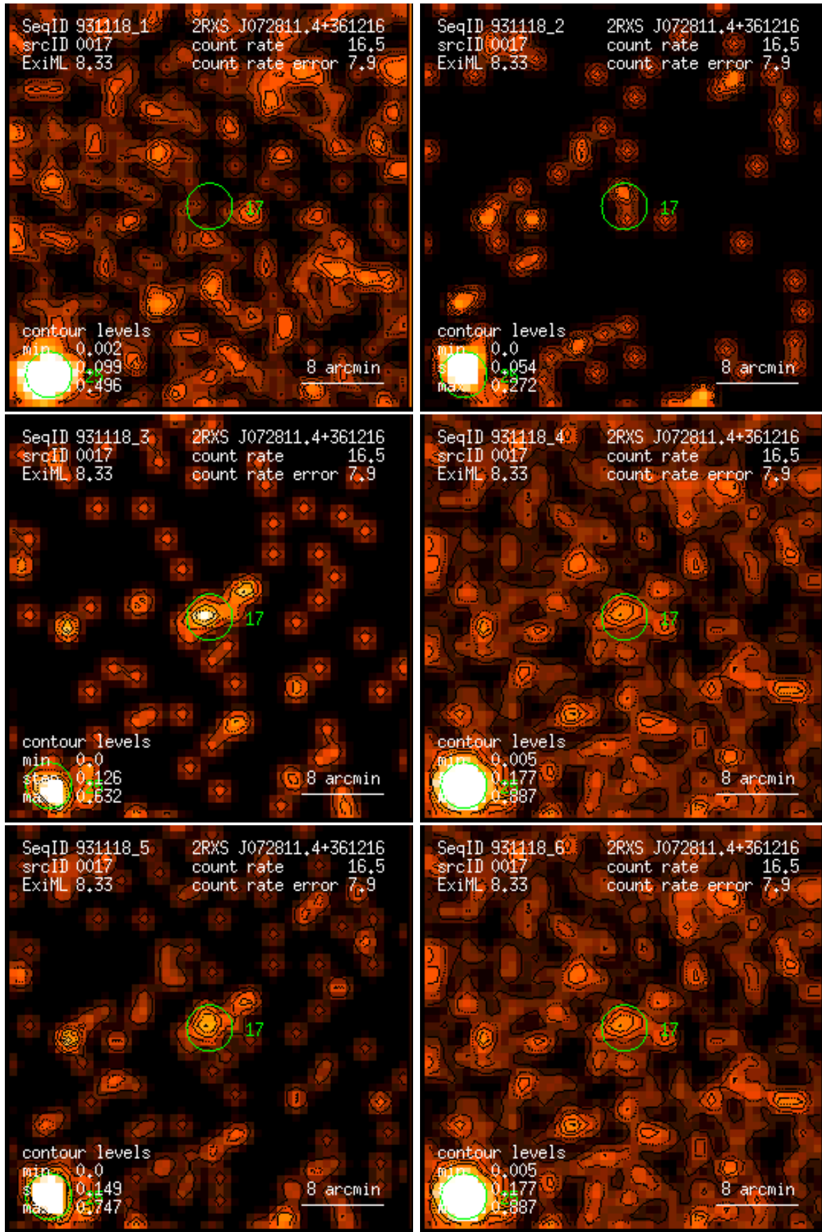
Figure 17: RASS 931118: detection 0017: band rate images, Gaussian filter: (1) PSPC channels 11 – 41, (2) 52 – 90, (3) 91 – 201, (4) 11 – 235, (5) 52 – 201, (6) 11 – 201. Broad band rates in counts/ks. Band rate contour levels in counts/ks/arcmin 2 .
