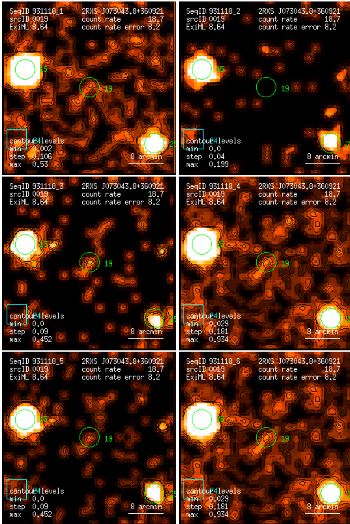
Figure 19: RASS 931118: detection 0019: band rate images, Gaussian filter: (1) PSPC channels 11 – 41, (2) 52 – 90, (3) 91 – 201, (4) 11 – 235, (5) 52 – 201, (6) 11 – 201. Broad band rates in counts/ks. Band rate contour levels in counts/ks/arcmin 2 .
