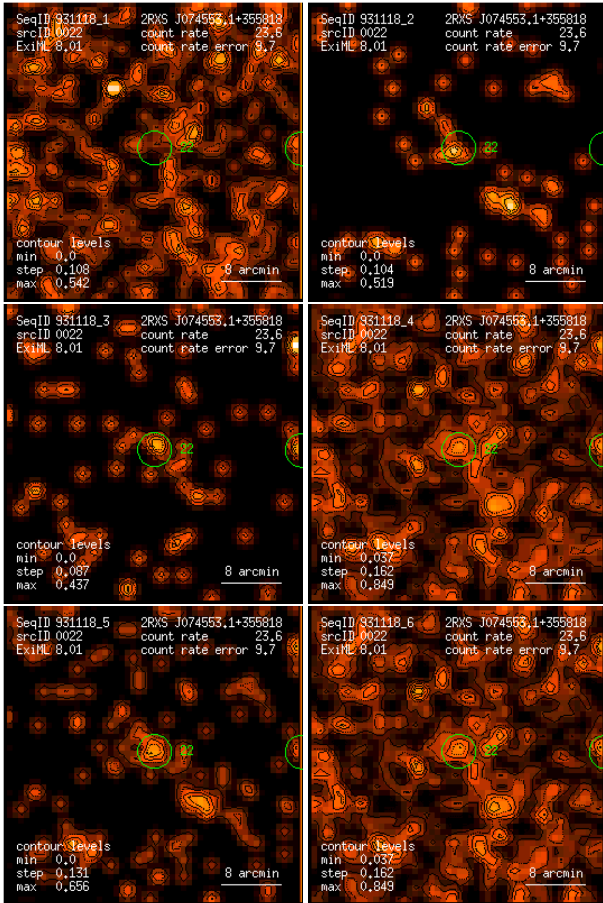
Figure 22: RASS 931118: detection 0022: band rate images, Gaussian filter: (1) PSPC channels 11 – 41, (2) 52 – 90, (3) 91 – 201, (4) 11 – 235, (5) 52 – 201, (6) 11 – 201. Broad band rates in counts/ks. Band rate contour levels in counts/ks/arcmin 2 .
