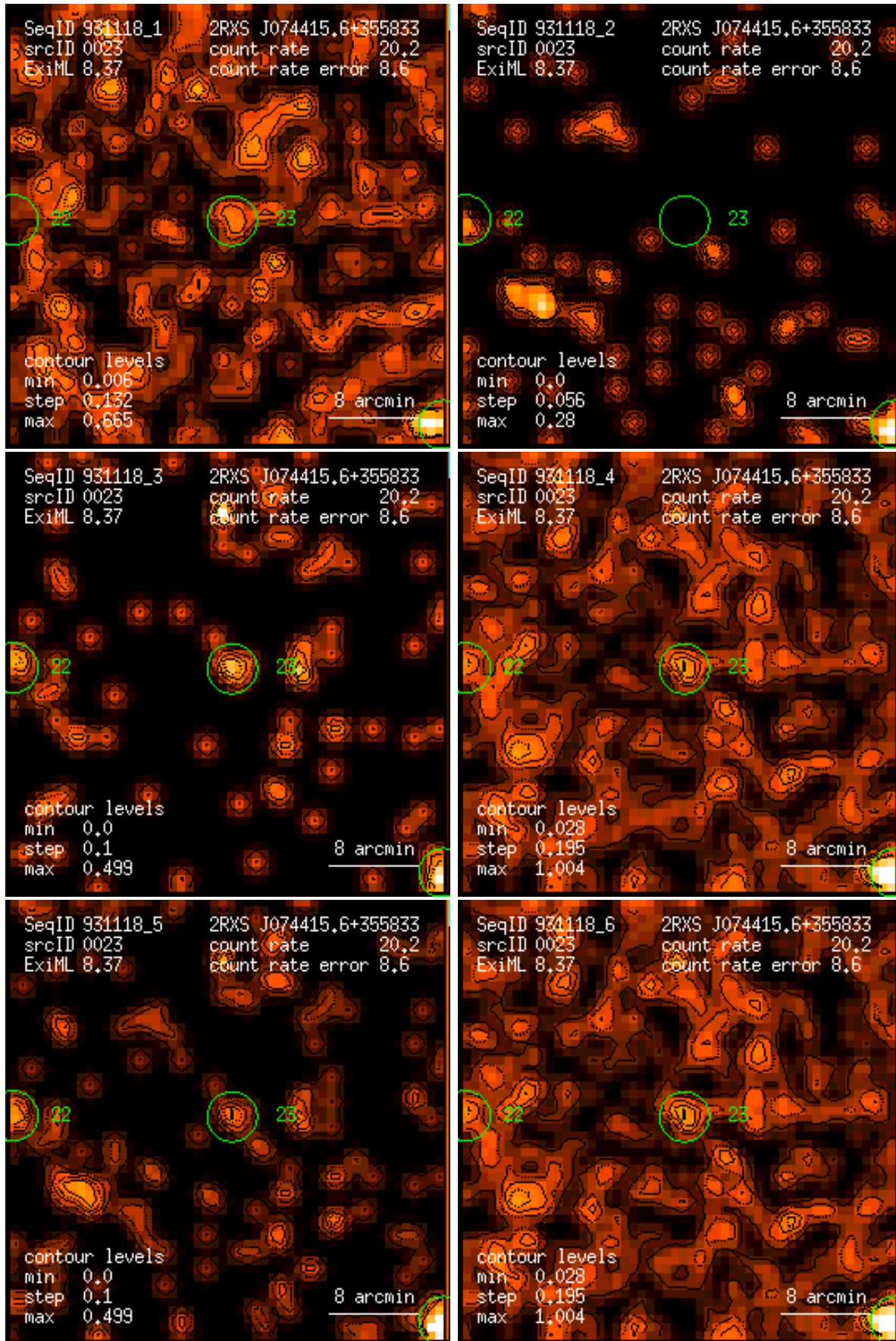
Figure 23: RASS 931118: detection 0023: band rate images, Gaussian filter: (1) PSPC channels 11 – 41, (2) 52 – 90, (3) 91 – 201, (4) 11 – 235, (5) 52 – 201, (6) 11 – 201. Broad band rates in counts/ks. Band rate contour levels in counts/ks/arcmin 2 .
