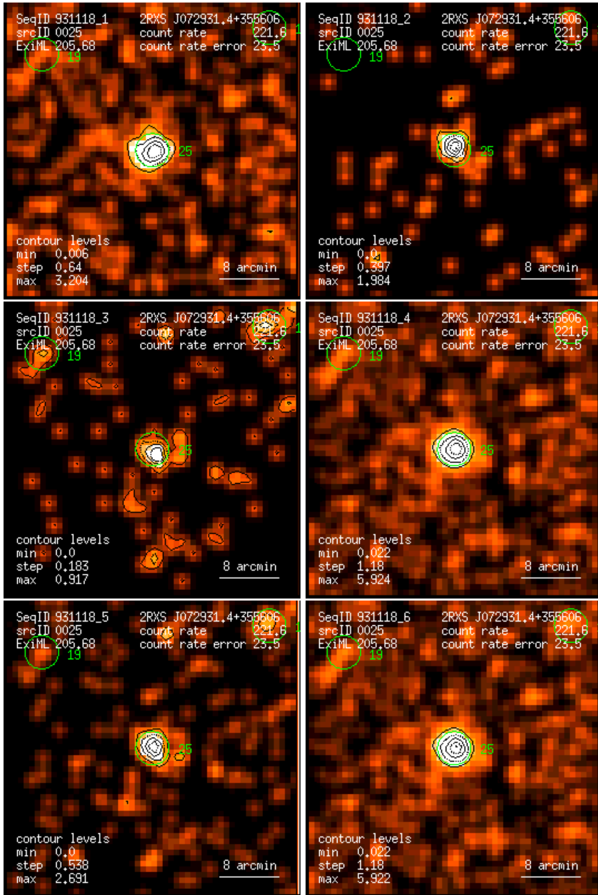
Figure 25: RASS 931118: detection 0025: band rate images, Gaussian filter: (1) PSPC channels 11 – 41, (2) 52 – 90, (3) 91 – 201, (4) 11 – 235, (5) 52 – 201, (6) 11 – 201. Broad band rates in counts/ks. Band rate contour levels in counts/ks/arcmin 2 .
