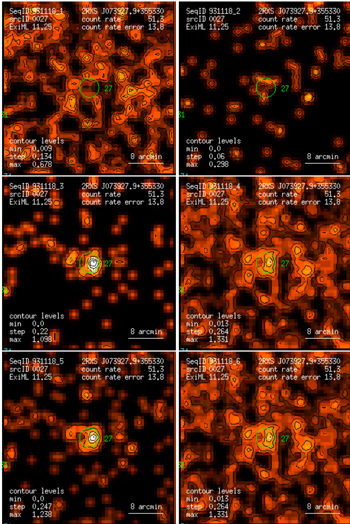
Figure 27: RASS 931118: detection 0027: band rate images, Gaussian filter: (1) PSPC channels 11 – 41, (2) 52 – 90, (3) 91 – 201, (4) 11 – 235, (5) 52 – 201, (6) 11 – 201. Broad band rates in counts/ks. Band rate contour levels in counts/ks/arcmin 2 .
