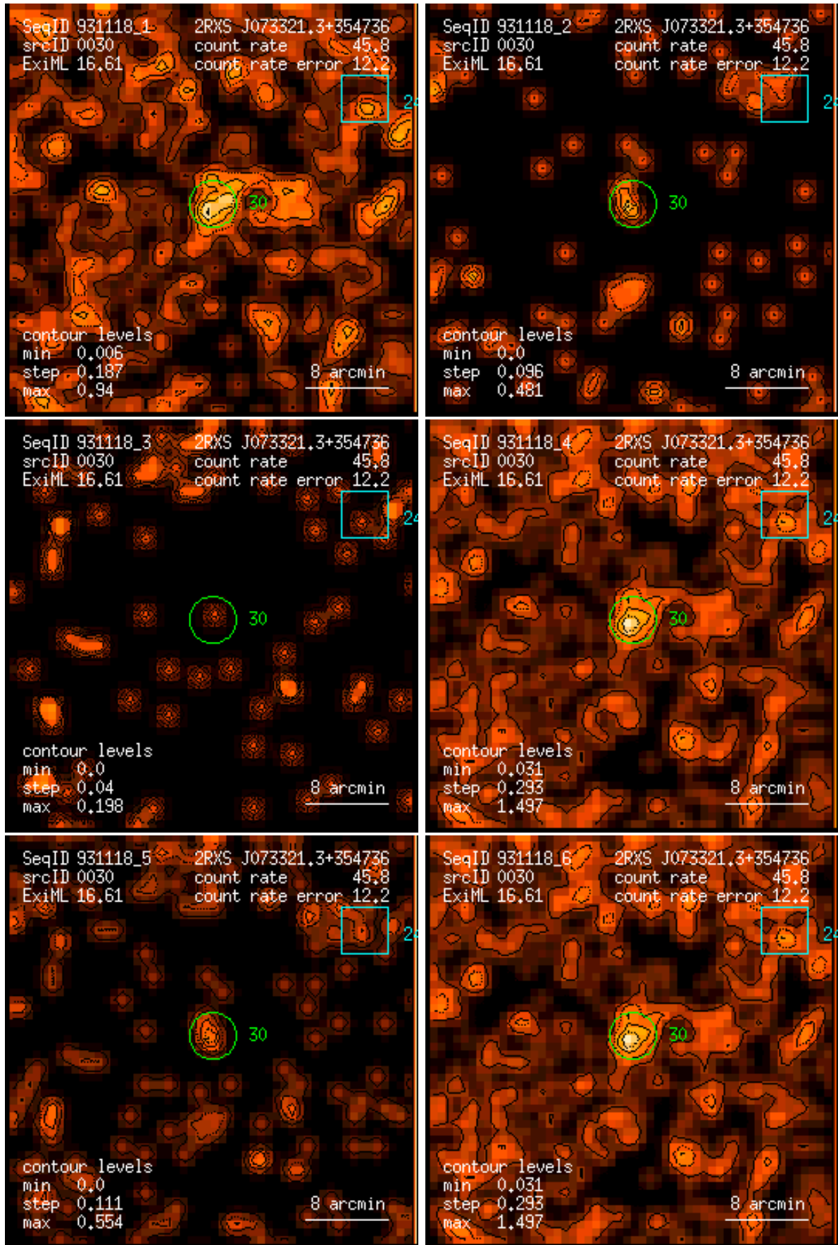
Figure 30: RASS 931118: detection 0030: band rate images, Gaussian filter: (1) PSPC channels 11 – 41, (2) 52 – 90, (3) 91 – 201, (4) 11 – 235, (5) 52 – 201, (6) 11 – 201. Broad band rates in counts/ks. Band rate contour levels in counts/ks/arcmin 2 .
