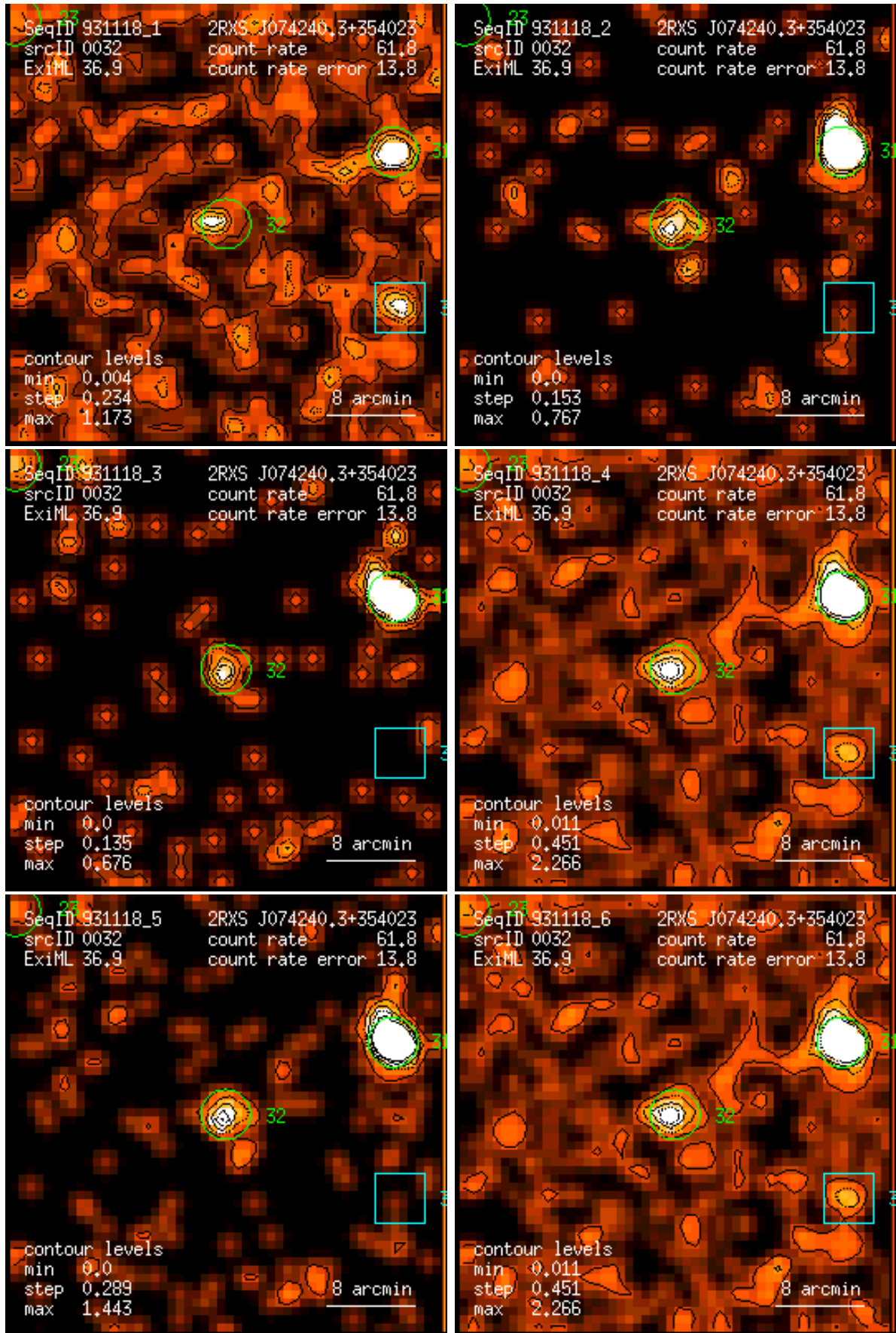
Figure 32: RASS 931118: detection 0032: band rate images, Gaussian filter: (1) PSPC channels 11 – 41, (2) 52 – 90, (3) 91 – 201, (4) 11 – 235, (5) 52 – 201, (6) 11 – 201. Broad band rates in counts/ks. Band rate contour levels in counts/ks/arcmin 2 .
