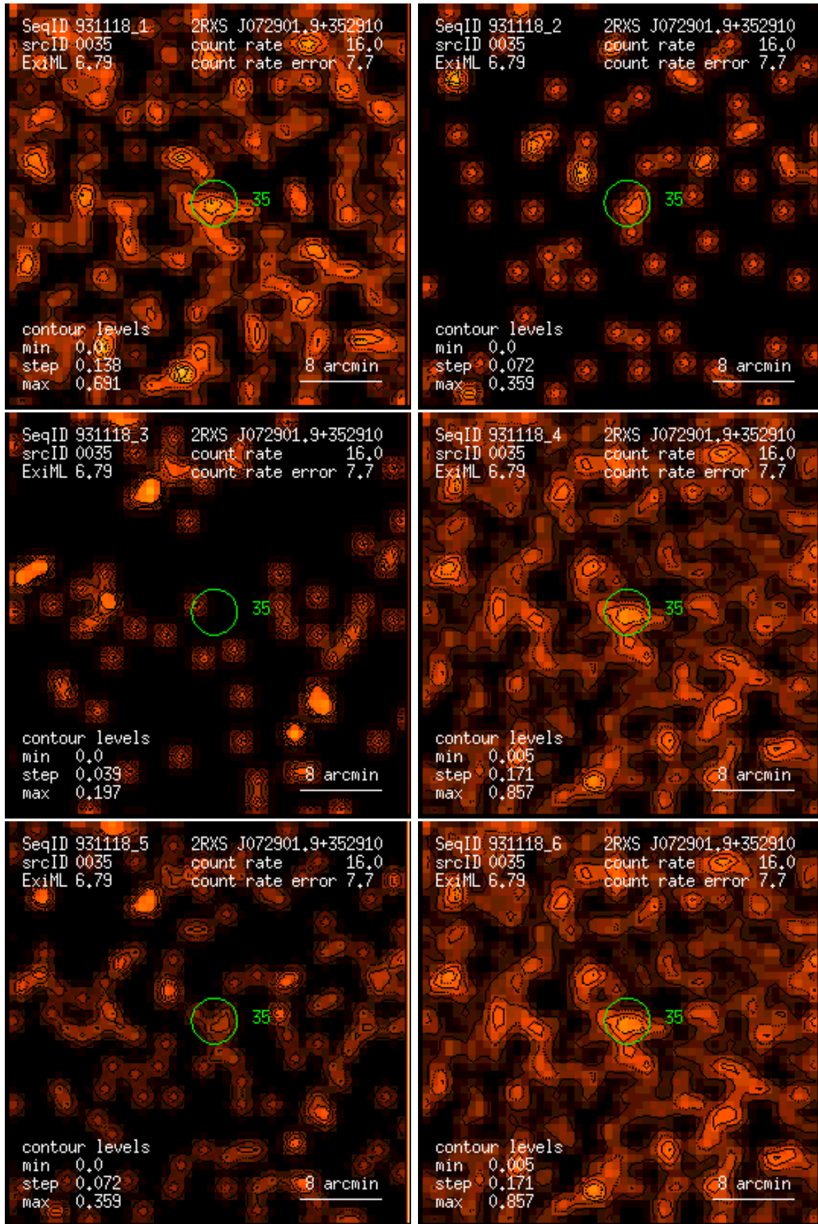
Figure 35: RASS 931118: detection 0035: band rate images, Gaussian filter: (1) PSPC channels 11 – 41, (2) 52 – 90, (3) 91 – 201, (4) 11 – 235, (5) 52 – 201, (6) 11 – 201. Broad band rates in counts/ks. Band rate contour levels in counts/ks/arcmin 2 .
