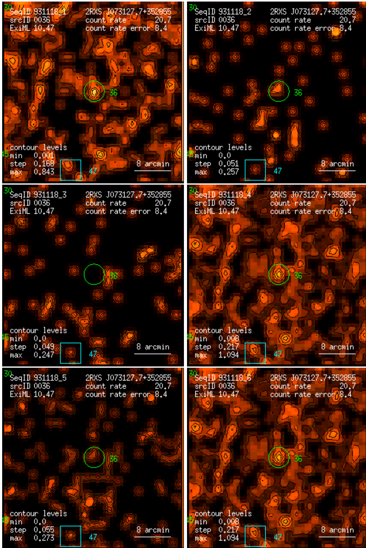
Figure 36: RASS 931118: detection 0036: band rate images, Gaussian filter: (1) PSPC channels 11 – 41, (2) 52 – 90, (3) 91 – 201, (4) 11 – 235, (5) 52 – 201, (6) 11 – 201. Broad band rates in counts/ks. Band rate contour levels in counts/ks/arcmin 2 .
