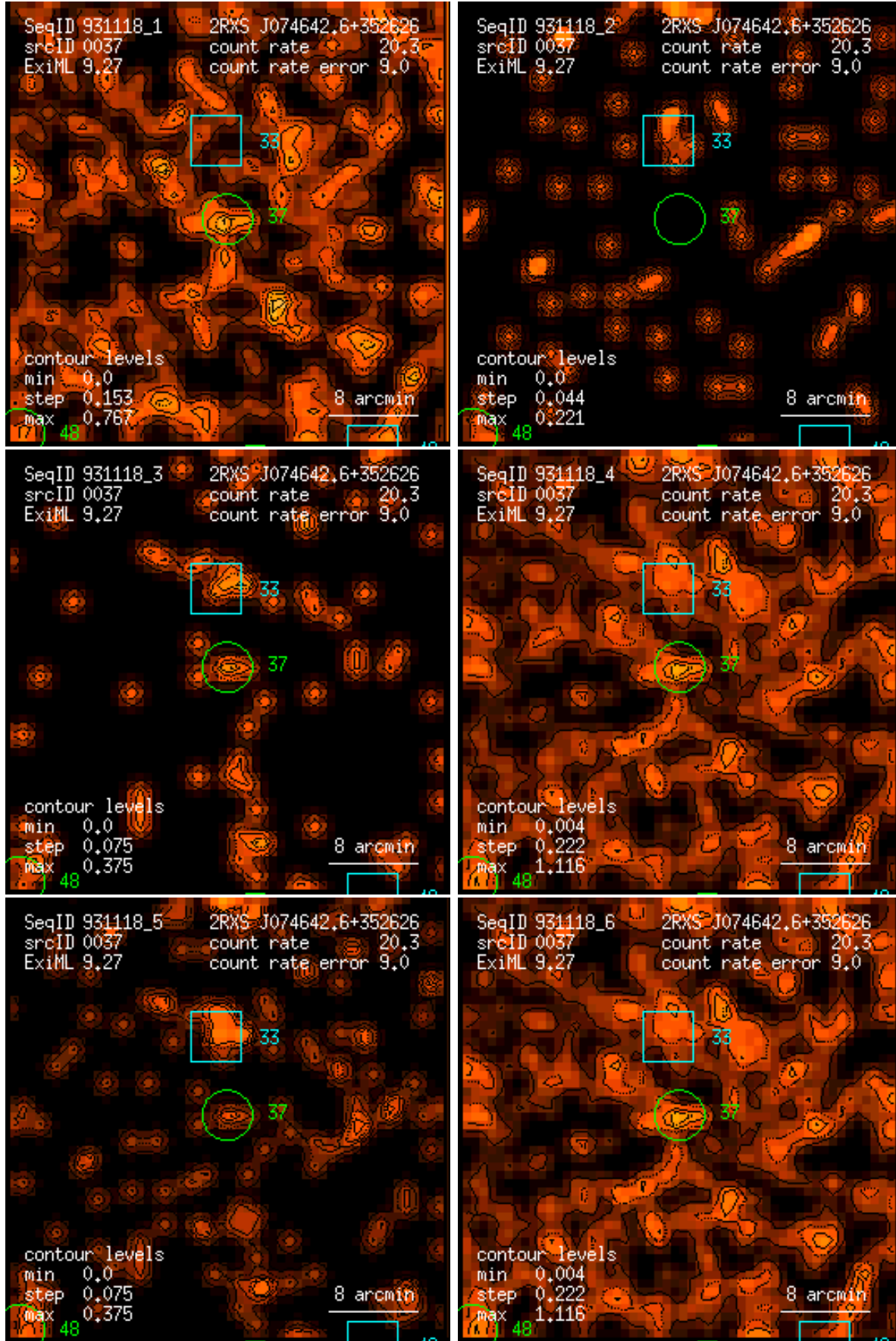
Figure 37: RASS 931118: detection 0037: band rate images, Gaussian filter: (1) PSPC channels 11 – 41, (2) 52 – 90, (3) 91 – 201, (4) 11 – 235, (5) 52 – 201, (6) 11 – 201. Broad band rates in counts/ks. Band rate contour levels in counts/ks/arcmin 2 .
