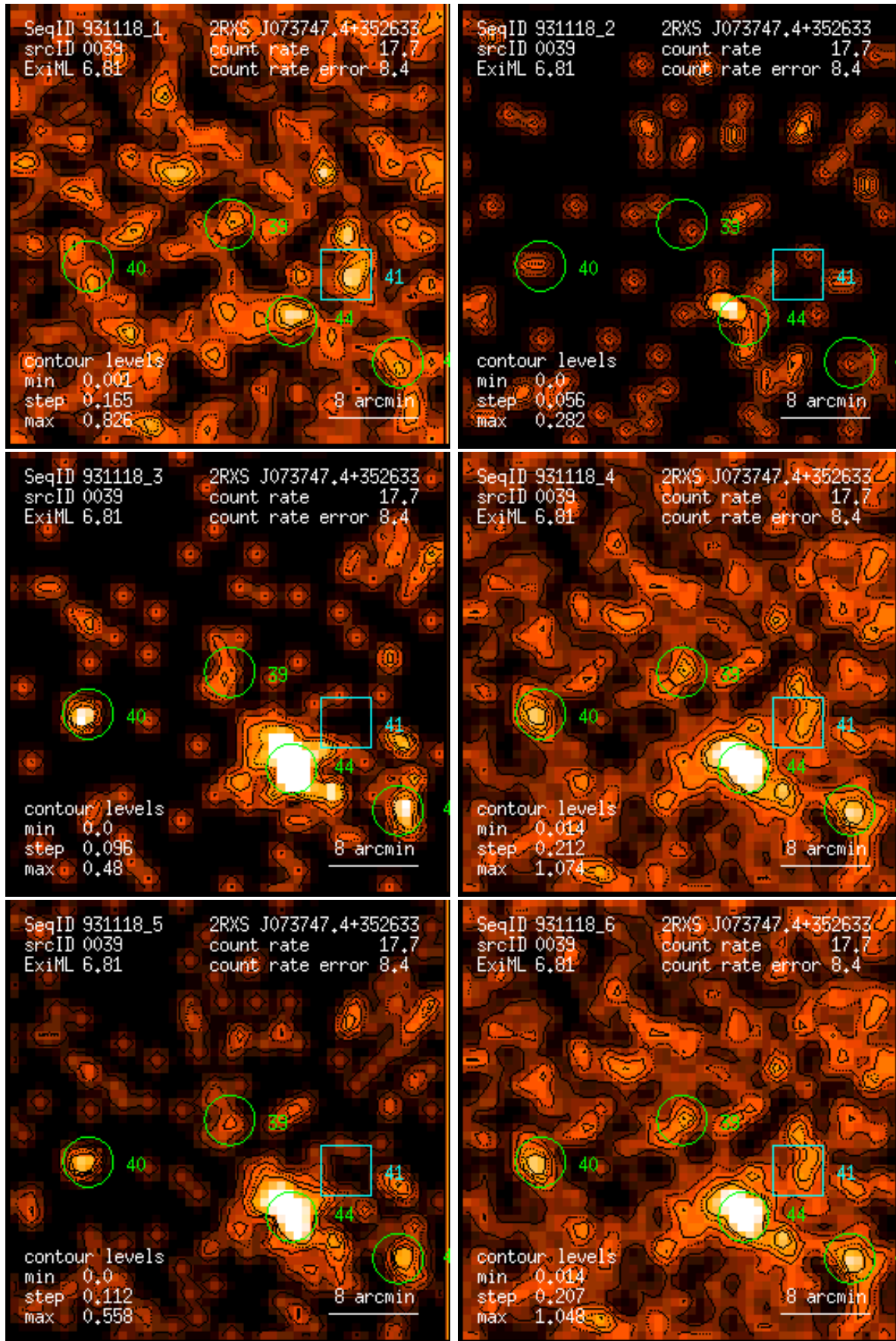
Figure 39: RASS 931118: detection 0039: band rate images, Gaussian filter: (1) PSPC channels 11 – 41, (2) 52 – 90, (3) 91 – 201, (4) 11 – 235, (5) 52 – 201, (6) 11 – 201. Broad band rates in counts/ks. Band rate contour levels in counts/ks/arcmin 2 .
