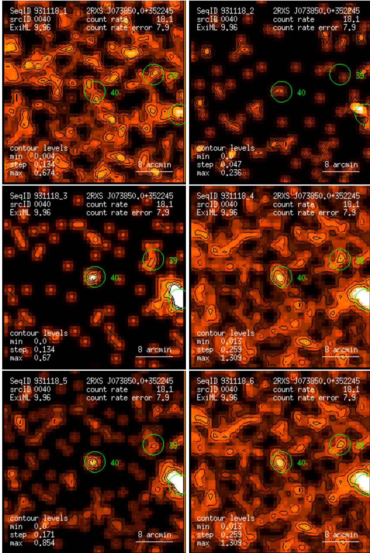
Figure 40: RASS 931118: detection 0040: band rate images, Gaussian filter: (1) PSPC channels 11 – 41, (2) 52 – 90, (3) 91 – 201, (4) 11 – 235, (5) 52 – 201, (6) 11 – 201. Broad band rates in counts/ks. Band rate contour levels in counts/ks/arcmin 2 .
