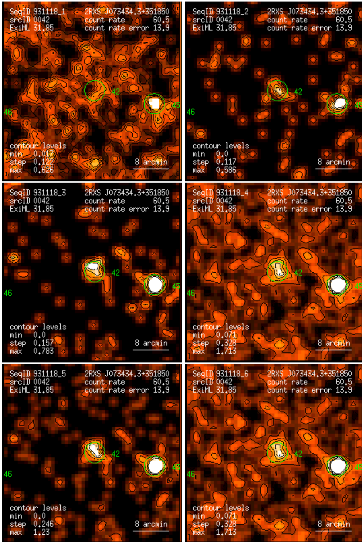
Figure 42: RASS 931118: detection 0042: band rate images, Gaussian filter: (1) PSPC channels 11 – 41, (2) 52 – 90, (3) 91 – 201, (4) 11 – 235, (5) 52 – 201, (6) 11 – 201. Broad band rates in counts/ks. Band rate contour levels in counts/ks/arcmin 2 .
