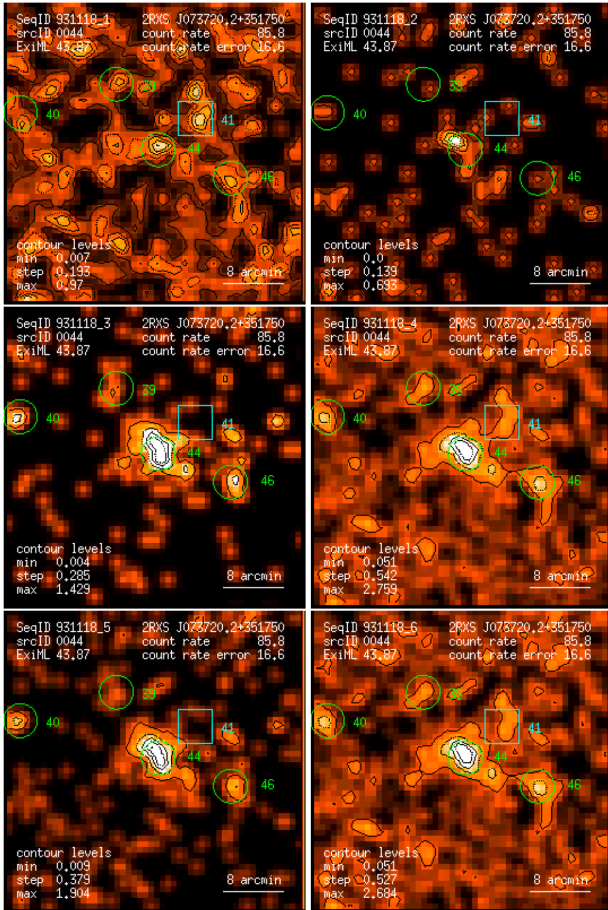
Figure 44: RASS 931118: detection 0044: band rate images, Gaussian filter: (1) PSPC channels 11 – 41, (2) 52 – 90, (3) 91 – 201, (4) 11 – 235, (5) 52 – 201, (6) 11 – 201. Broad band rates in counts/ks. Band rate contour levels in counts/ks/arcmin 2 .
