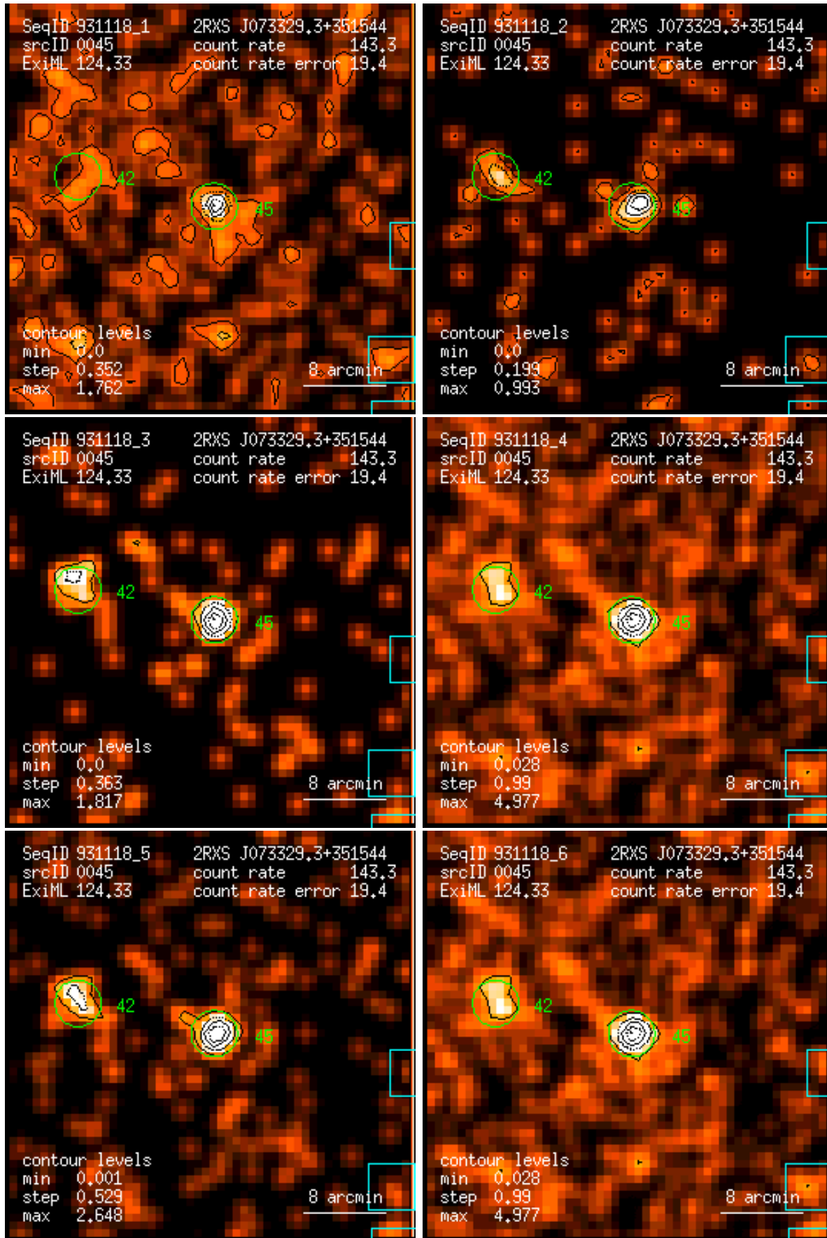
Figure 45: RASS 931118: detection 0045: band rate images, Gaussian filter: (1) PSPC channels 11 – 41, (2) 52 – 90, (3) 91 – 201, (4) 11 – 235, (5) 52 – 201, (6) 11 – 201. Broad band rates in counts/ks. Band rate contour levels in counts/ks/arcmin 2 .
