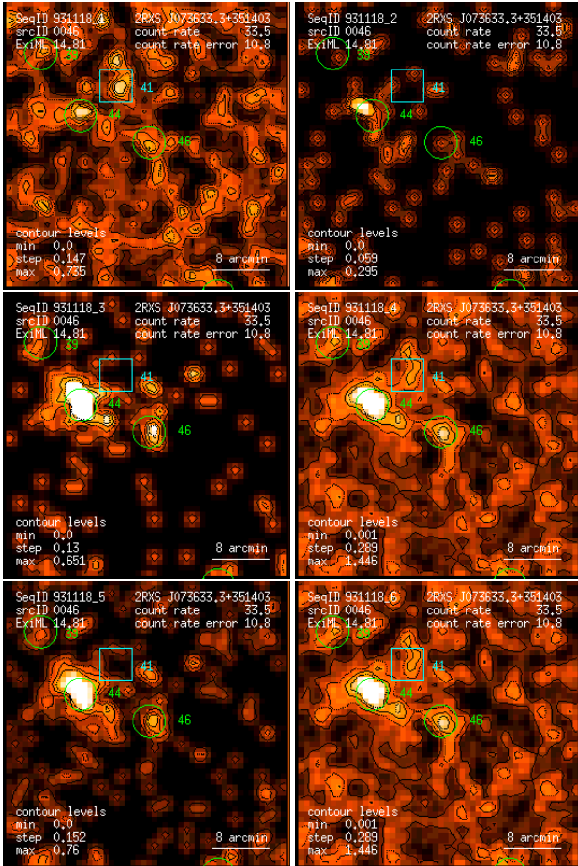
Figure 46: RASS 931118: detection 0046: band rate images, Gaussian filter: (1) PSPC channels 11 – 41, (2) 52 – 90, (3) 91 – 201, (4) 11 – 235, (5) 52 – 201, (6) 11 – 201. Broad band rates in counts/ks. Band rate contour levels in counts/ks/arcmin 2 .
