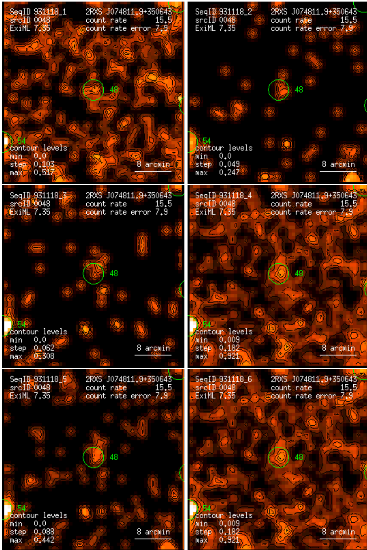
Figure 48: RASS 931118: detection 0048: band rate images, Gaussian filter: (1) PSPC channels 11 – 41, (2) 52 – 90, (3) 91 – 201, (4) 11 – 235, (5) 52 – 201, (6) 11 – 201. Broad band rates in counts/ks. Band rate contour levels in counts/ks/arcmin 2 .
