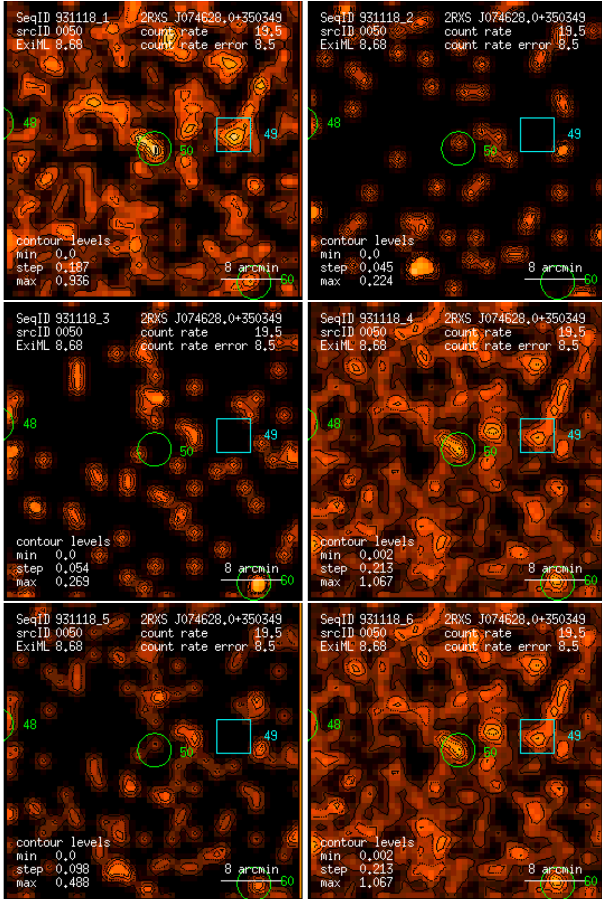
Figure 50: RASS 931118: detection 0050: band rate images, Gaussian filter: (1) PSPC channels 11 – 41, (2) 52 – 90, (3) 91 – 201, (4) 11 – 235, (5) 52 – 201, (6) 11 – 201. Broad band rates in counts/ks. Band rate contour levels in counts/ks/arcmin 2 .
