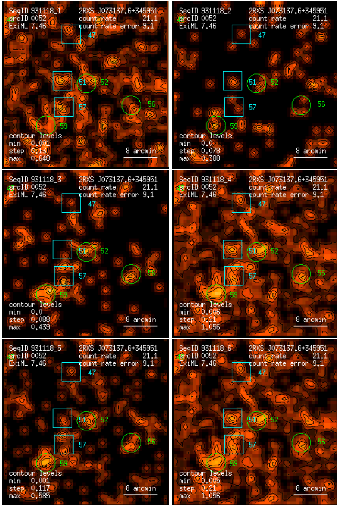
Figure 52: RASS 931118: detection 0052: band rate images, Gaussian filter: (1) PSPC channels 11 – 41, (2) 52 – 90, (3) 91 – 201, (4) 11 – 235, (5) 52 – 201, (6) 11 – 201. Broad band rates in counts/ks. Band rate contour levels in counts/ks/arcmin 2 .
