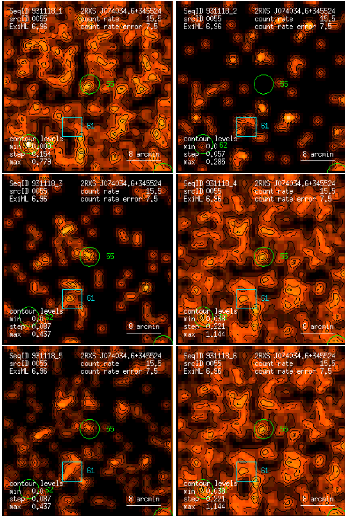
Figure 55: RASS 931118: detection 0055: band rate images, Gaussian filter: (1) PSPC channels 11 – 41, (2) 52 – 90, (3) 91 – 201, (4) 11 – 235, (5) 52 – 201, (6) 11 – 201. Broad band rates in counts/ks. Band rate contour levels in counts/ks/arcmin 2 .
