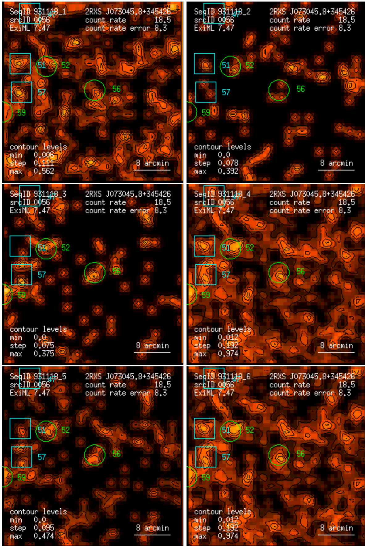
Figure 56: RASS 931118: detection 0056: band rate images, Gaussian filter: (1) PSPC channels 11 – 41, (2) 52 – 90, (3) 91 – 201, (4) 11 – 235, (5) 52 – 201, (6) 11 – 201. Broad band rates in counts/ks. Band rate contour levels in counts/ks/arcmin 2 .
