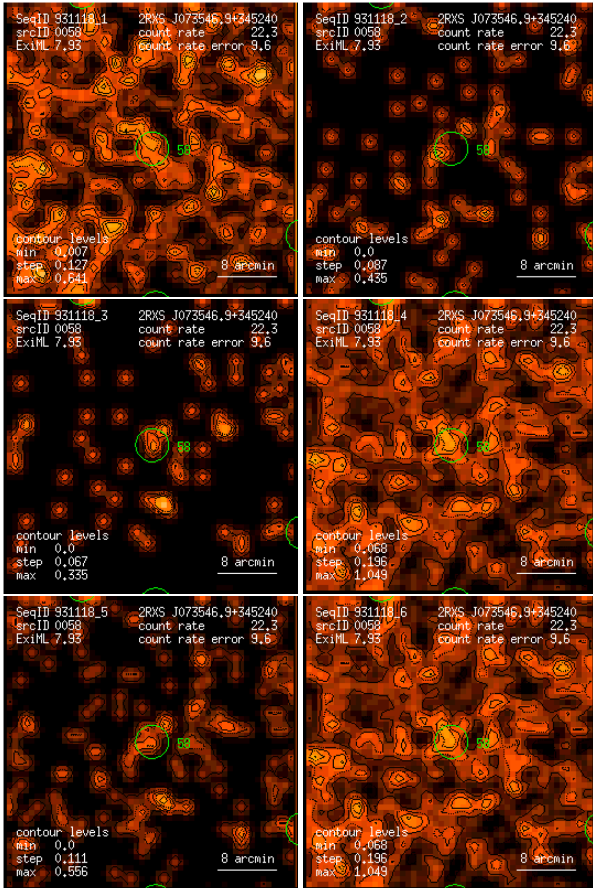
Figure 58: RASS 931118: detection 0058: band rate images, Gaussian filter: (1) PSPC channels 11 – 41, (2) 52 – 90, (3) 91 – 201, (4) 11 – 235, (5) 52 – 201, (6) 11 – 201. Broad band rates in counts/ks. Band rate contour levels in counts/ks/arcmin 2 .
