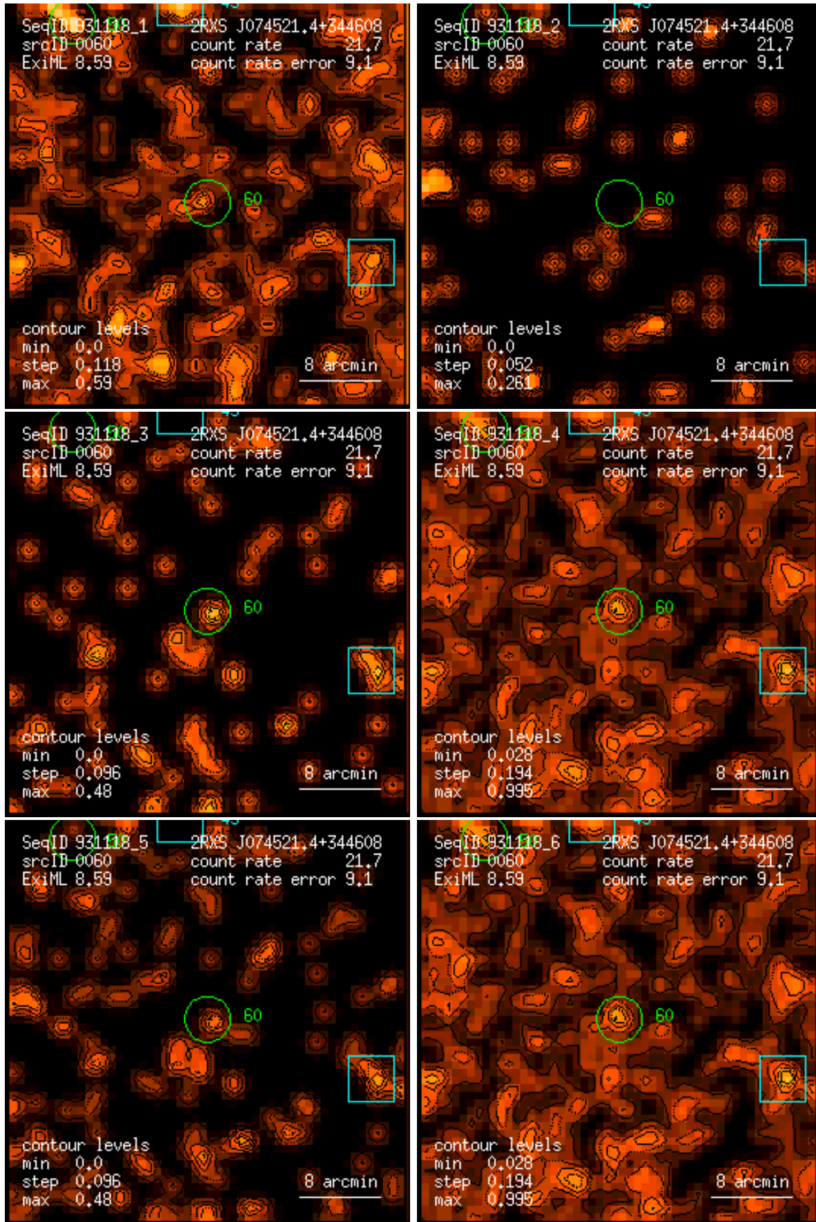
Figure 60: RASS 931118: detection 0060: band rate images, Gaussian filter: (1) PSPC channels 11 – 41, (2) 52 – 90, (3) 91 – 201, (4) 11 – 235, (5) 52 – 201, (6) 11 – 201. Broad band rates in counts/ks. Band rate contour levels in counts/ks/arcmin 2 .
