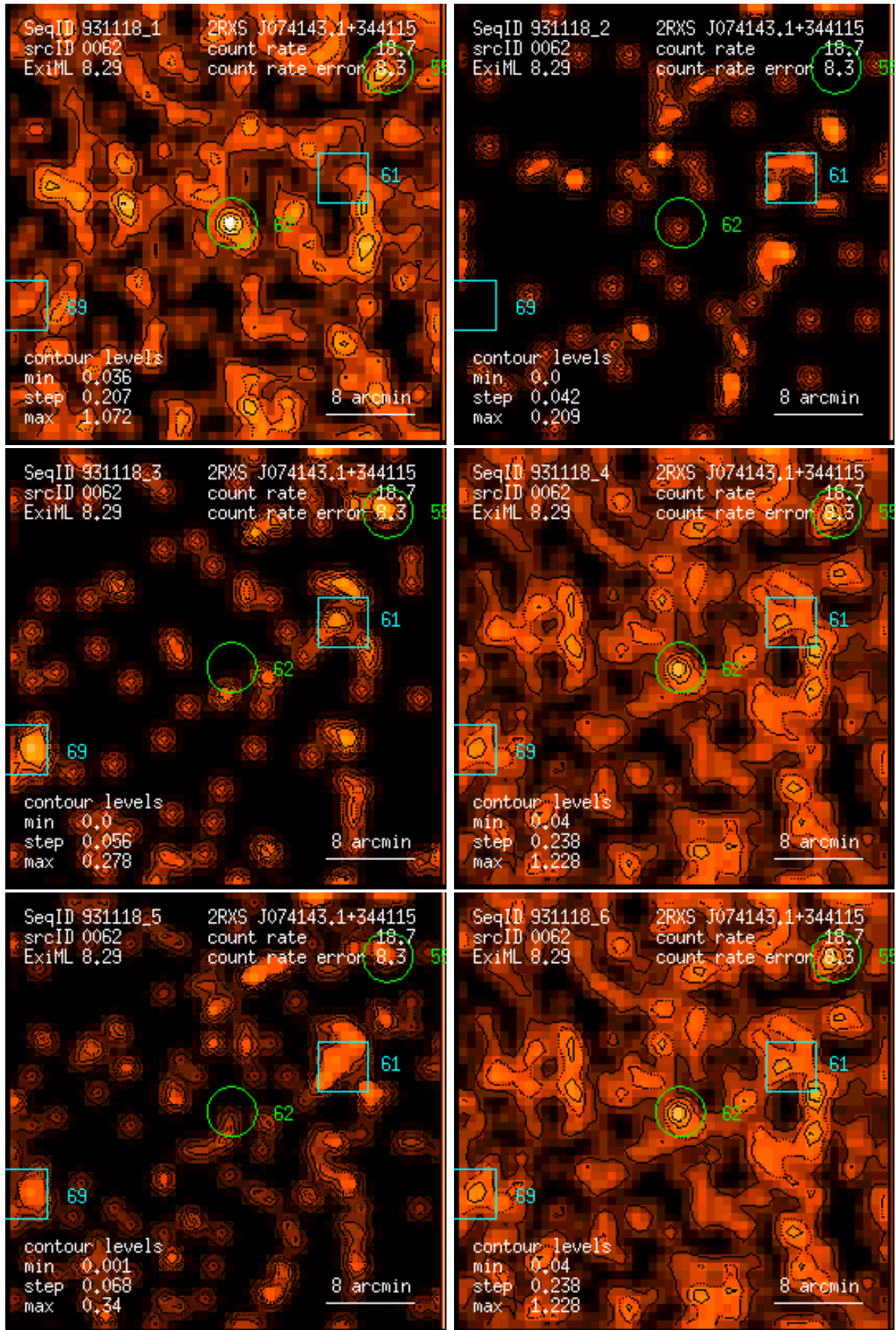
Figure 62: RASS 931118: detection 0062: band rate images, Gaussian filter: (1) PSPC channels 11 – 41, (2) 52 – 90, (3) 91 – 201, (4) 11 – 235, (5) 52 – 201, (6) 11 – 201. Broad band rates in counts/ks. Band rate contour levels in counts/ks/arcmin 2 .
