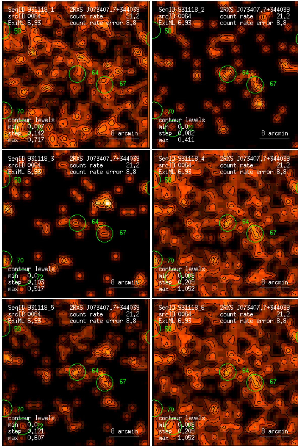
Figure 64: RASS 931118: detection 0064: band rate images, Gaussian filter: (1) PSPC channels 11 – 41, (2) 52 – 90, (3) 91 – 201, (4) 11 – 235, (5) 52 – 201, (6) 11 – 201. Broad band rates in counts/ks. Band rate contour levels in counts/ks/arcmin 2 .
