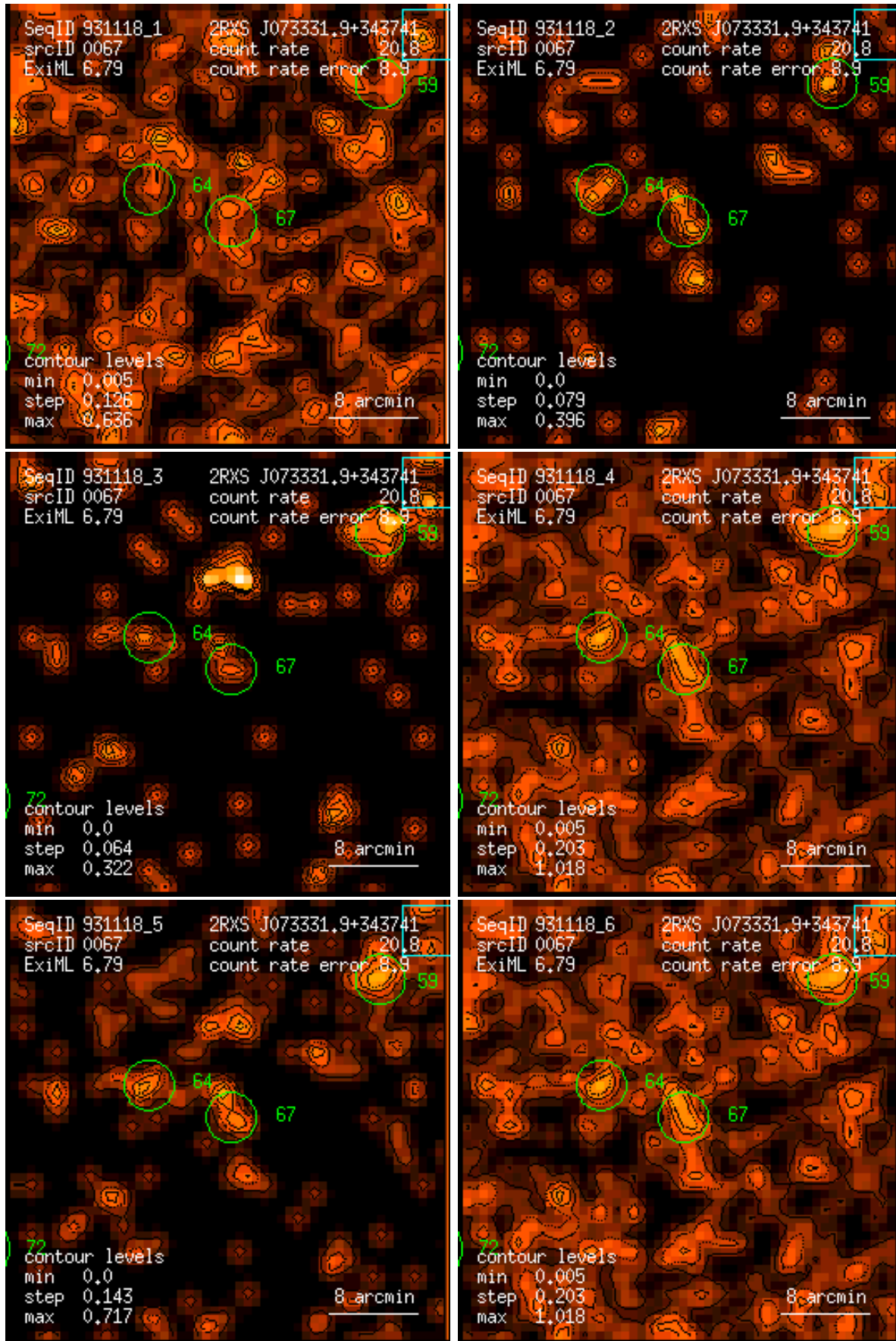
Figure 67: RASS 931118: detection 0067: band rate images, Gaussian filter: (1) PSPC channels 11 – 41, (2) 52 – 90, (3) 91 – 201, (4) 11 – 235, (5) 52 – 201, (6) 11 – 201. Broad band rates in counts/ks. Band rate contour levels in counts/ks/arcmin 2 .
