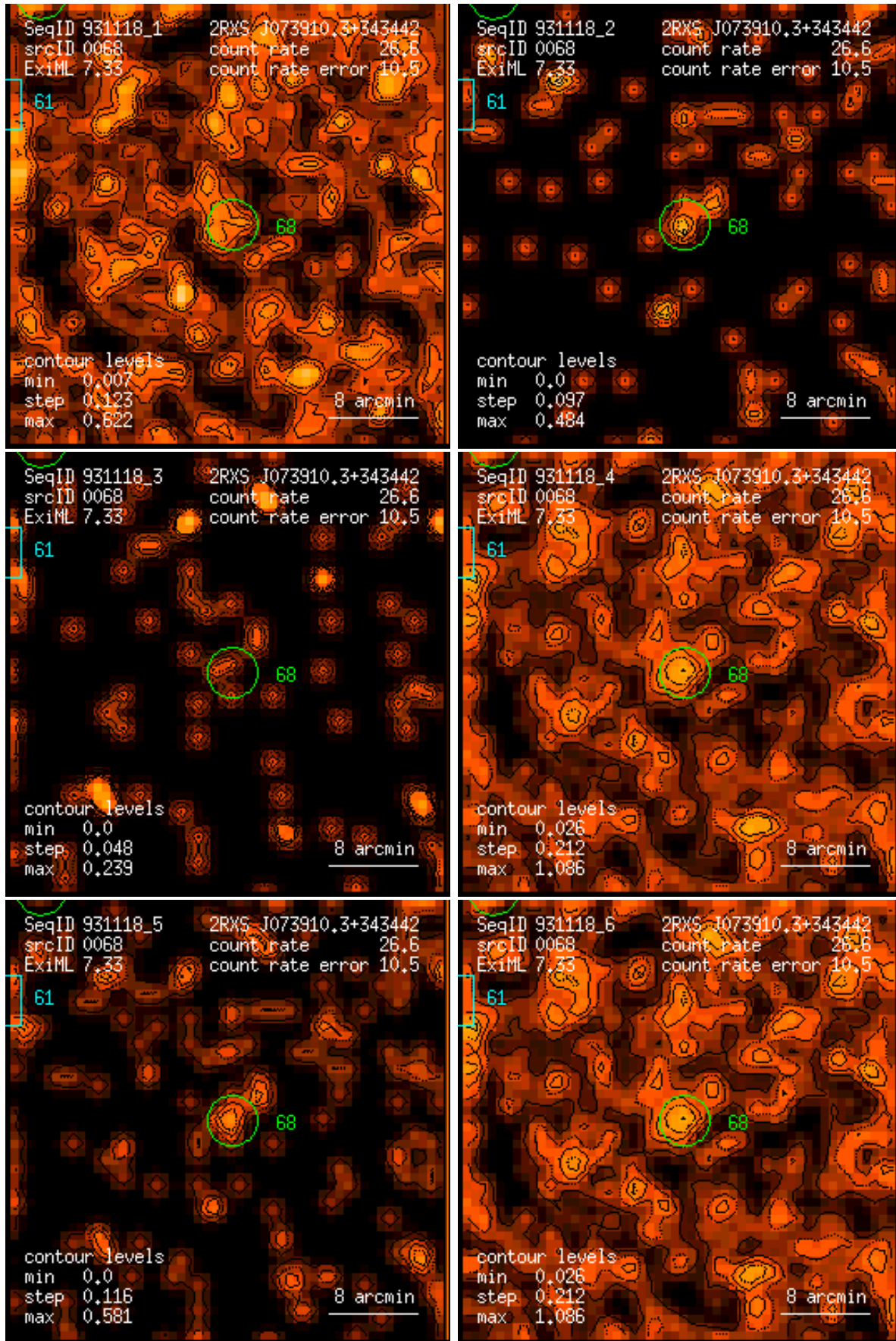
Figure 68: RASS 931118: detection 0068: band rate images, Gaussian filter: (1) PSPC channels 11 – 41, (2) 52 – 90, (3) 91 – 201, (4) 11 – 235, (5) 52 – 201, (6) 11 – 201. Broad band rates in counts/ks. Band rate contour levels in counts/ks/arcmin 2 .
