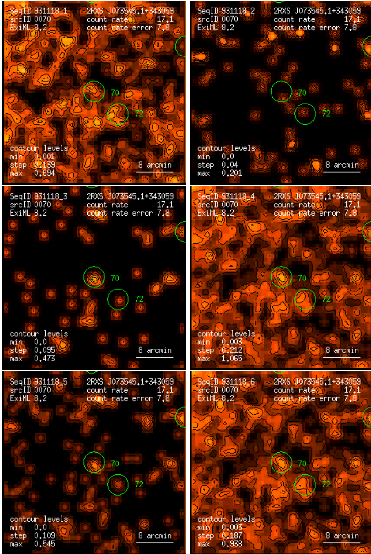
Figure 70: RASS 931118: detection 0070: band rate images, Gaussian filter: (1) PSPC channels 11 – 41, (2) 52 – 90, (3) 91 – 201, (4) 11 – 235, (5) 52 – 201, (6) 11 – 201. Broad band rates in counts/ks. Band rate contour levels in counts/ks/arcmin 2 .
