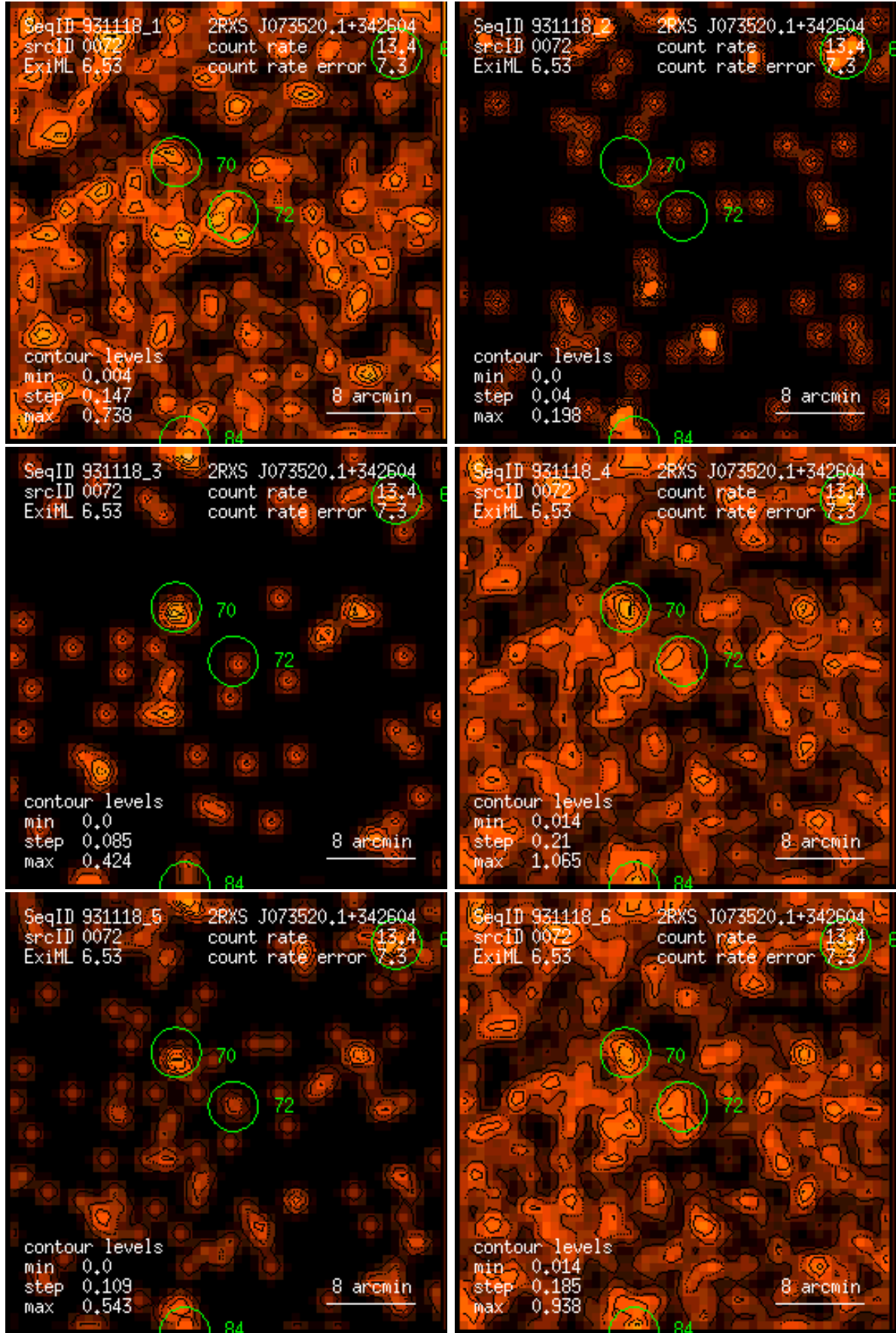
Figure 72: RASS 931118: detection 0072: band rate images, Gaussian filter: (1) PSPC channels 11 – 41, (2) 52 – 90, (3) 91 – 201, (4) 11 – 235, (5) 52 – 201, (6) 11 – 201. Broad band rates in counts/ks. Band rate contour levels in counts/ks/arcmin 2 .
