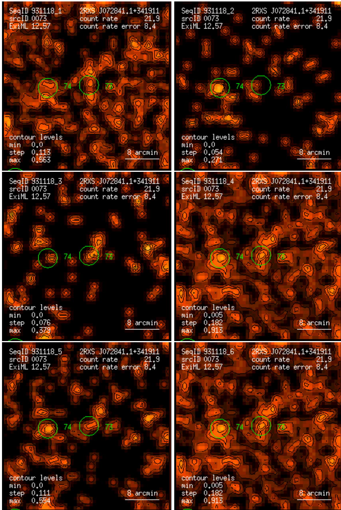
Figure 73: RASS 931118: detection 0073: band rate images, Gaussian filter: (1) PSPC channels 11 – 41, (2) 52 – 90, (3) 91 – 201, (4) 11 – 235, (5) 52 – 201, (6) 11 – 201. Broad band rates in counts/ks. Band rate contour levels in counts/ks/arcmin 2 .
