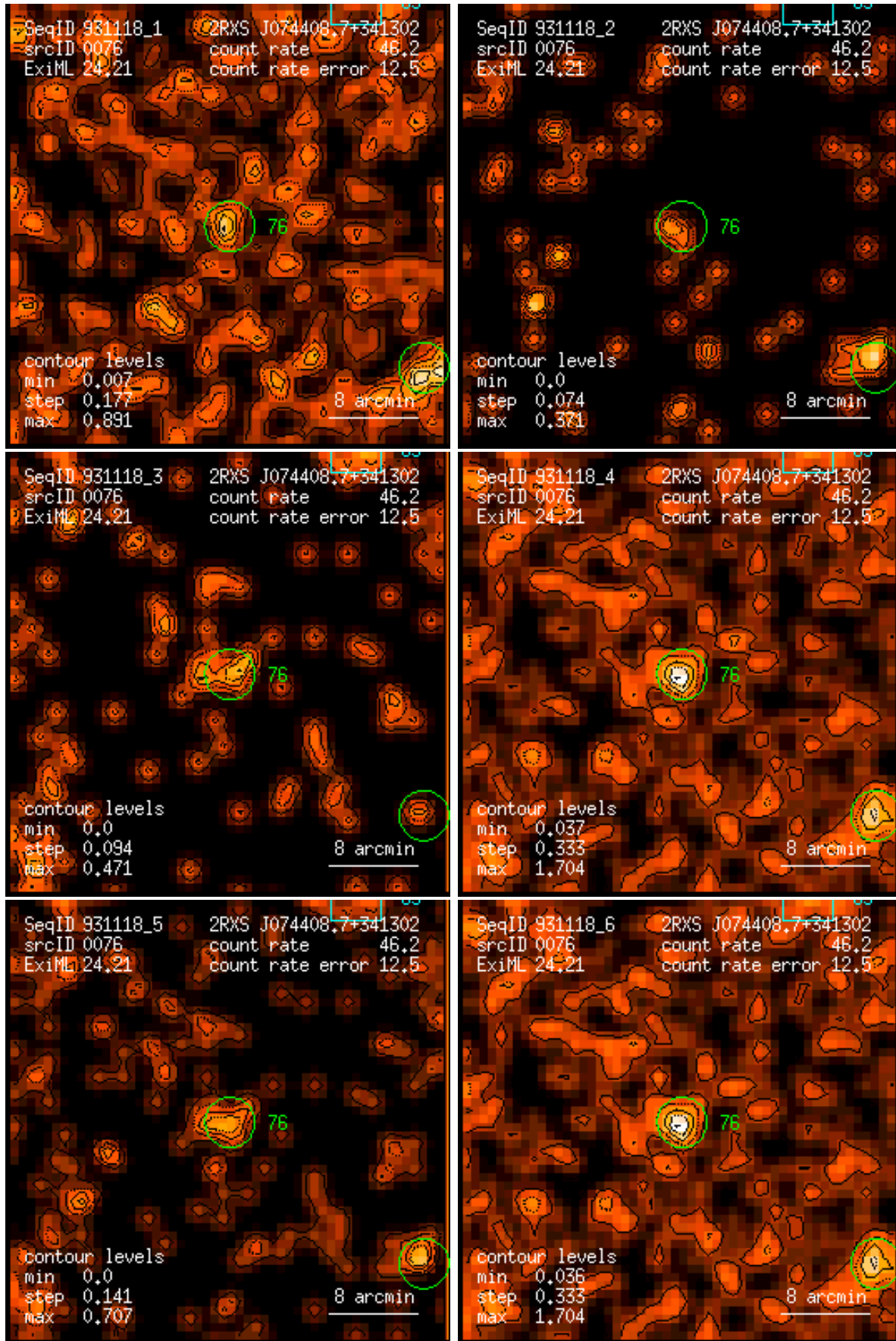
Figure 76: RASS 931118: detection 0076: band rate images, Gaussian filter: (1) PSPC channels 11 – 41, (2) 52 – 90, (3) 91 – 201, (4) 11 – 235, (5) 52 – 201, (6) 11 – 201. Broad band rates in counts/ks. Band rate contour levels in counts/ks/arcmin 2 .
