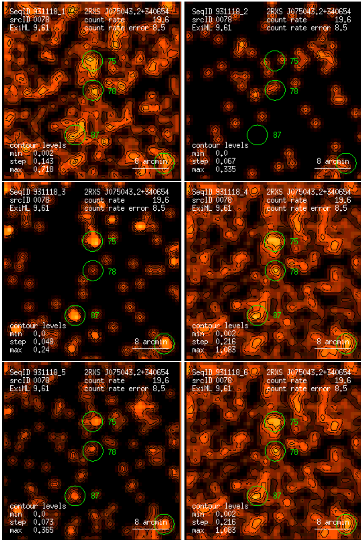
Figure 78: RASS 931118: detection 0078: band rate images, Gaussian filter: (1) PSPC channels 11 – 41, (2) 52 – 90, (3) 91 – 201, (4) 11 – 235, (5) 52 – 201, (6) 11 – 201. Broad band rates in counts/ks. Band rate contour levels in counts/ks/arcmin 2 .
