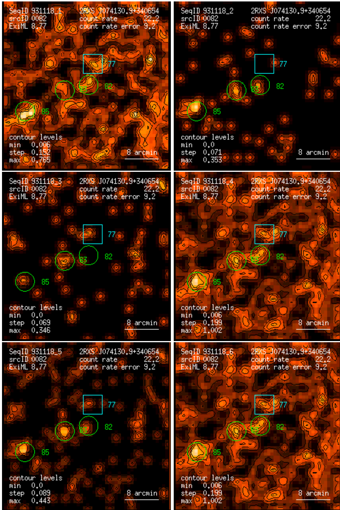
Figure 82: RASS 931118: detection 0082: band rate images, Gaussian filter: (1) PSPC channels 11 – 41, (2) 52 – 90, (3) 91 – 201, (4) 11 – 235, (5) 52 – 201, (6) 11 – 201. Broad band rates in counts/ks. Band rate contour levels in counts/ks/arcmin 2 .
